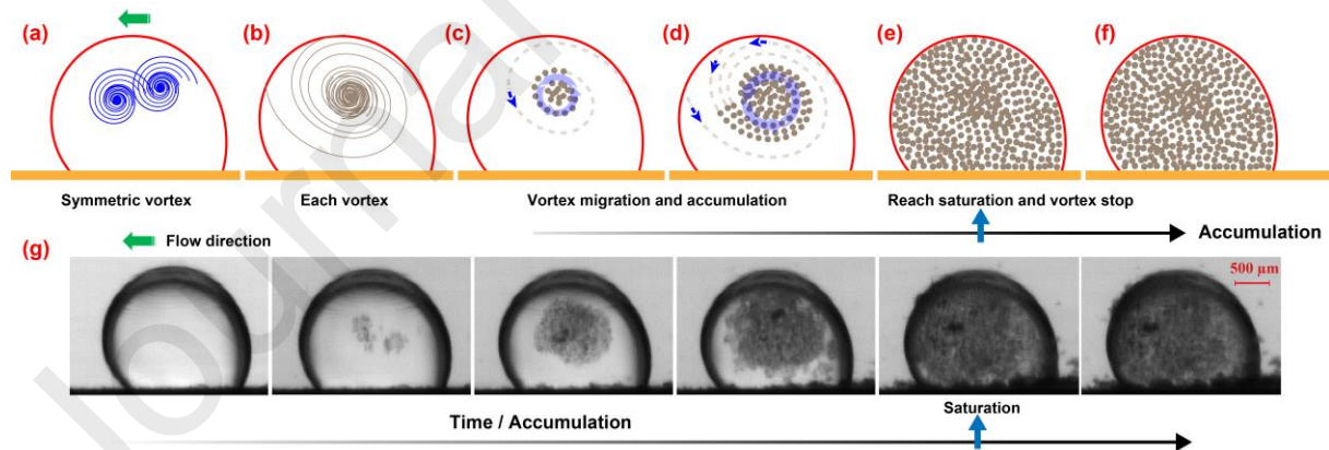
Fig. 4. Influence of internal circulation on particle capture process. (a) Symmetric vortex. There are two symmetric vortices inside the droplet, so it can be assumed that the droplet could be divided into two symmetric parts. (b) Particle migration. The particles captured from the vortex edge will be continuously carried into the vortex core by internal circulation. (c-e)
