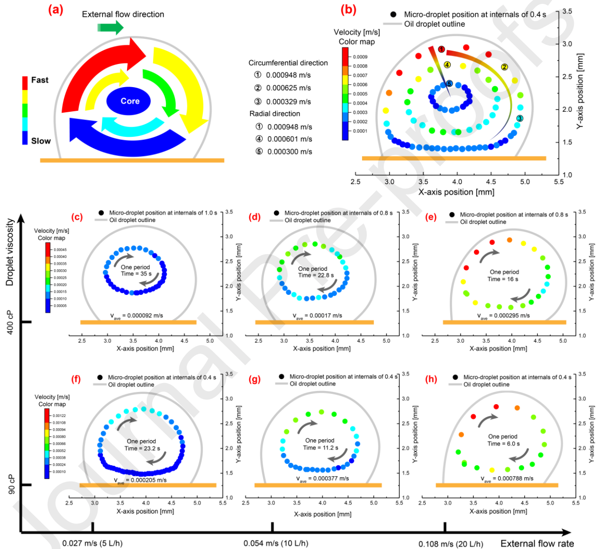
Fig. 1. Internal circulation and velocity distribution. (a) The whole droplet is rotated, and the center of rotation is a low-velocity vortex core region. The velocity on the windward side is the fastest, and then it attenuates in both the circumferential and radial directions. (b) The velocity distribution at different streamline positions demonstrates the mode of velocity attenuation.
