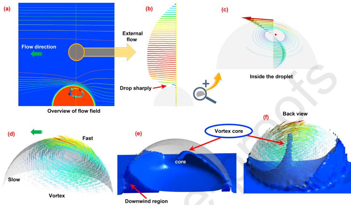
Fig. 2. Comprehensive flow pattern. (a) Overall external flow field in the channel. In the channel, the external flow field is laminar, and the adhered droplet acts as an obstacle. When the external fluid passes around the droplet, it has the maximum velocity gradient (streamlines are the densest) in the area close to the upper part of the windward side, while it is almost stationary in the area behind the leeward side of the droplet. (b) The velocity distribution on a vertical line (the yellow line from (a)) passing through the droplet. The length and direction of the line represent the relative magnitude and direction of the velocity. The external flow velocity has a parabolic distribution, and it drops sharply when approaching the droplet interface. Compared with the external flow velocity, the velocity within the droplet is too small, so that the velocity line inside the droplet is barely visible. (c) Local relative velocity distribution inside the droplet. Local magnification of the droplet (from (b)) shows the local
