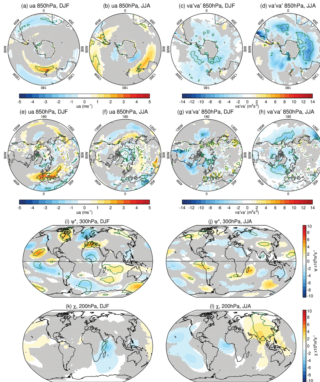
Figure A1. CMIP6 ensemble mean bias relative to ERA5. Gray shading depicts regions where less than 75% of the models agree on the sign of the bias and green contour shows where more than 95% of the models agree on the sign of the bias. (a, b, e, and f) The 850-hPa u_a . (c, d, g, and h) The 850-hPa 10-day high-pass eddy meridional wind variance. (i and j) The 300-hPa eddy stream function; (k and l) the 200-hPa velocity potential.
