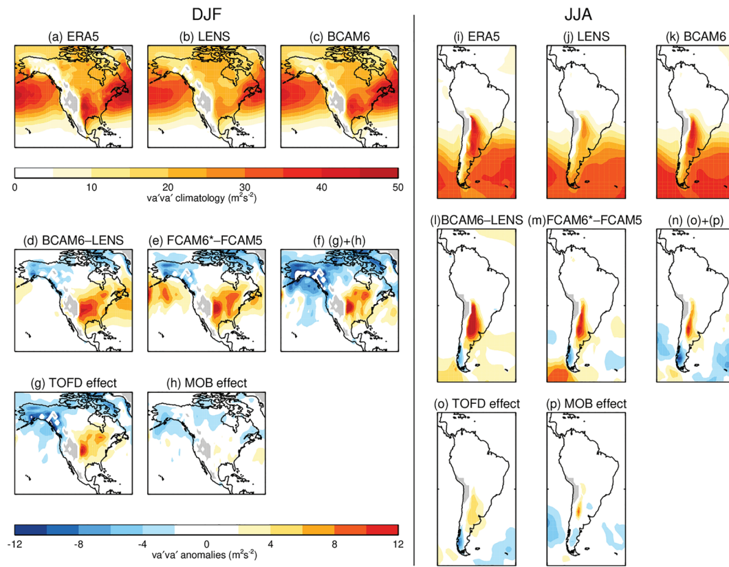
Figure 7. Ten-day high-pass-filtered meridional wind variance \overline{v'v'} in the lee of the Rockies (left columns) and the Andes (right columns) during winter. For the Rockies, panels (a)–(c) show the climatologies for ERA5, LENS, and BCAM6. (d) The BCAM6-LENS that can be compared with panel (e), which shows the FCAM6* – FCAM5 difference that forms the baseline for the sensitivity tests. (f) The sum of the differences FCAM6* – FCAM6_TMS and FCAM6* – FCAM6_NOMOB, that is, the influences of the TOFD and MOB schemes inferred by reverting them back to CAM5 settings. The individual differences FCAM6* – FCAM6_TMS and FCAM6* – FCAM6_NOMOB can be seen in panels (g) and (h). Panels (i)–(p) are as in (a)–(h) but over South America during JJA. Gray regions are where the 850-hPa level lies below the surface.
