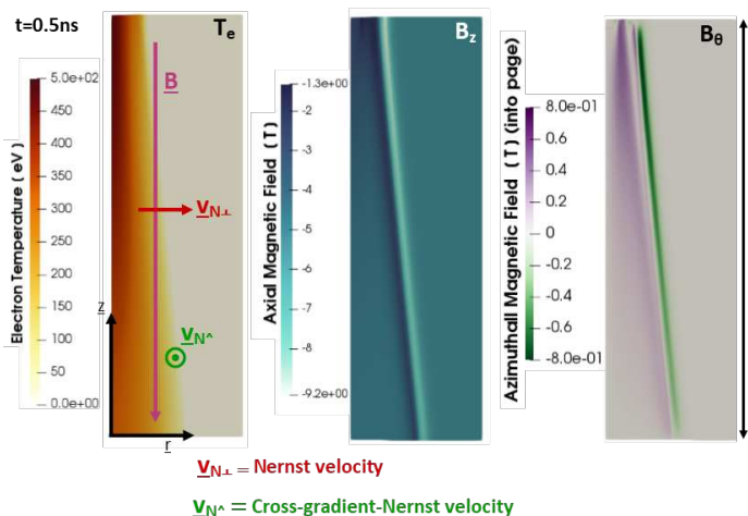
FIG. 4. Electron temperature and axial/azimuthal magnetic field components for the cross-gradient-Nernst configuration. Along the labelled magnetic field line the cross-gradient-Nernst moves out of the page at low Z and is zero at high Z , resulting in a twisted field component.
