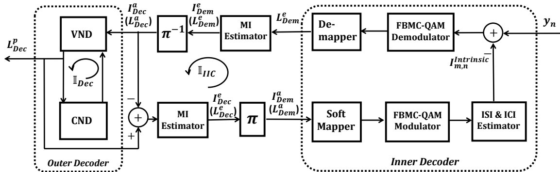
Fig. 4: IIC-based BICM-ID system model for EXIT Chart analysis
