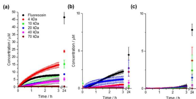
Figure 2. Concentration of fluorophores at the base of gels of dimension 1 cm \times 1 cm \times 0.5 cm (height). Diffusion through (a) DBS-CONH 2 (6 mM, 0.285% wt/vol) (b) the hybrid gel consisting of DBS-CONH 2 (6 mM, 0.285% wt/vol) and PEGDM (10% wt/vol) and (c) PEGDM (10% wt/vol) hydrogels. Errors given as standard deviation ( n = 3 ).
