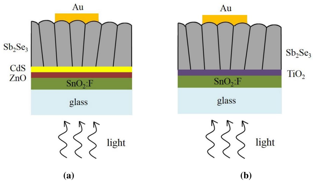
Figure 1. Schematic illustration of (a) \text{Sb}_2\text{Se}_3 -CdS and (b) \text{Sb}_2\text{Se}_3 - \text{TiO}_2 device structures.
