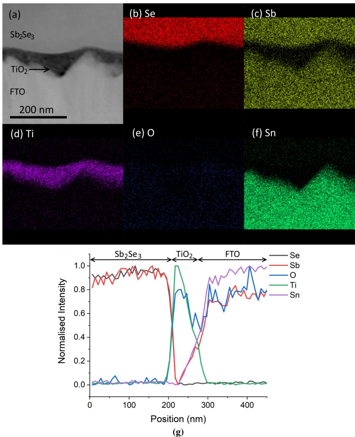
Figure 9. EDX chemical maps acquired across the \text{Sb}_2\text{Se}_3 - \text{TiO}_2 interface in the close space sublimated \text{Sb}_2\text{Se}_3 - \text{TiO}_2 sample. The STEM bright field image is shown in (a) with the individual layers labelled (FTO denotes fluorine doped \text{SnO}_2 ). EDX maps for Se, Sb, Ti, O and Sn are shown in (b)-(f) respectively. An EDX linescan from a different region is plotted
