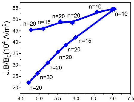
1 (a) \alpha (Normalized pressure gradient) (b) J.B/B_0 versus \alpha_{ped} 2 Figure 4. Peeling-ballooning boundary of CFETR R=6.6m phase II in (a) J.B/B_0 versus \alpha_{ped} 3 space obtained from density scan in EPED , and (b) J.B/B_0 versus pedestal height space. The 4 density is scaled by 10^{19} \text{ m}^{-3} .
