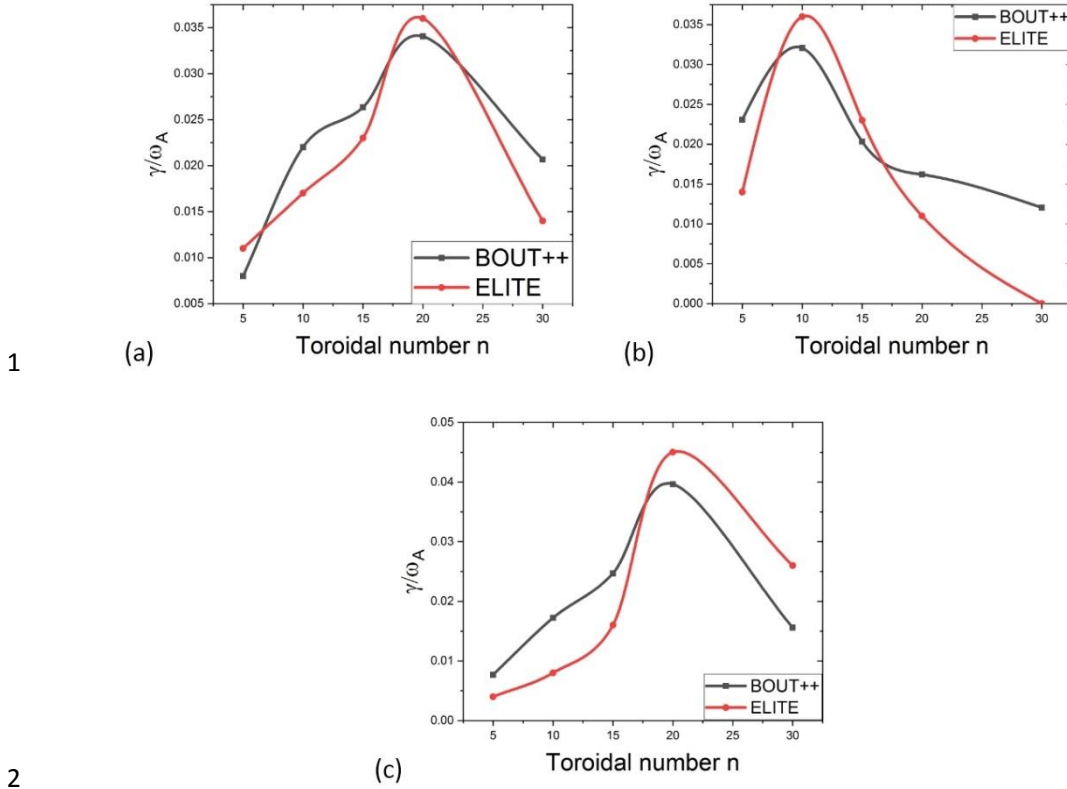
3 Figure 7. Unstable mode spectrum computed by BOUT++ at (a) low collisionality ( v^*=0.14 ), 4 (b) intermediate collisionality ( v^*=0.39 ) and (c) high collisionality ( v^*=1.31 ). The black curves 5 are from BOUT++ and the red curves are from ELITE.
