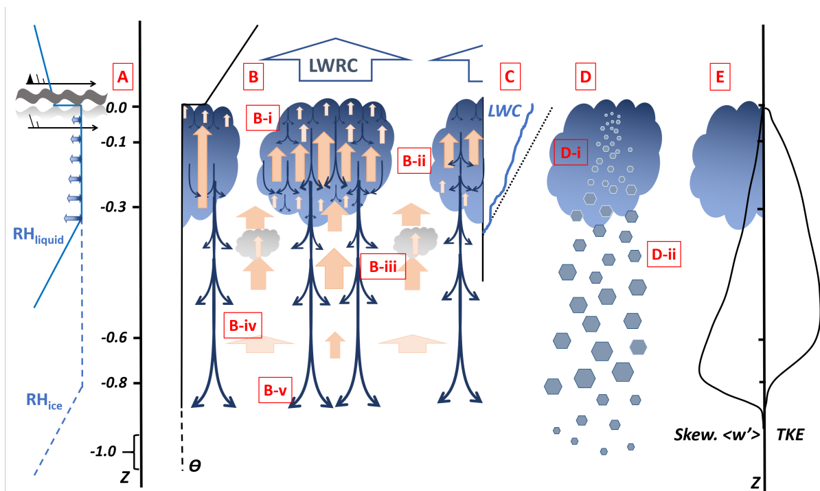
Figure 13. Schematic of processes that control altocumulus clouds as a function of normalised cloud layer depth below cloud top altitude, Z . The lower boundary is typically diffuse unlike for stratocumulus - which has the surface as a lower boundary (a) cloud formation through wind shear or gravity wave activity acting at a stable interface in potential temperature, ( \theta - black trace) with a suitable relative humidity distribution (blue solid - RH w.r.t. liquid, and blue dashed - RH w.r.t. ice, and arrows indicate distribution up to 100 % )just below the temperature inversion. (b) Clouds (blue parcels) cool through Long-wave radiative cooling from cloud top, a process which imparts turbulence to the layer below with narrow strong downdrafts (blue arrows) and broad weaker updrafts (red arrows). (b-i) to (b-v) see text for details of the resulting turbulence structure (c) Turbulence acts to maintain the liquid water content profile (blue line) in a pseudo-adiabatic form (dashed black line). (d) At temperatures lower than 0^{\circ}\text{C} , ice nucleation may occur, located within the liquid cloud, resulting in ice precipitating from the liquid cloud layer. (e) Turbulence Kinetic Energy peak occurs below the liquid cloud layer, with the skewness of the vertical velocity distribution occurring lower still.
