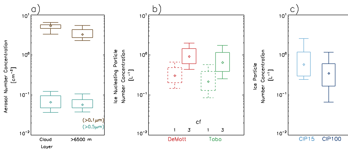
Figure 12. (a) Percentiles of aerosol particle number concentrations larger than 0.1 \mu\text{m} (brown) and 0.5 \mu\text{m} (teal) from PCASP for the cloud layer (left) and above 6500 m (right). (b) INP concentrations [ \text{L}^{-1} ] using DeMott et al. (2015) (red), and Tobo et al. (2013) (green) with INC correction factors (DeMott et al., 2015) of 1 (dashed) and 3 (solid). (c) Ice Particle number concentrations N_i from CIP15 (light blue) and CIP100 (dark blue).
