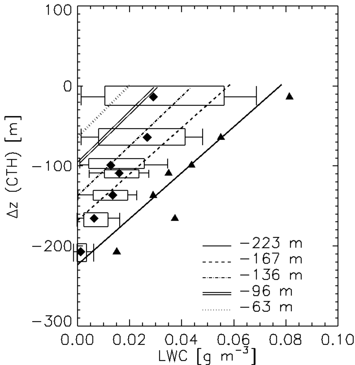
Figure 8. LWC profile relative to CTH for the mixed-phase cloud layer with data from Nevzorov LWC sensor. Theoretical profiles show adiabatic ascents of saturated air parcels. The ascents begin at the mean altitude of the statistics box levels, apart from for the base layer which begins at the bottom of the level. See legend for details. Statistics as Fig. 4.
