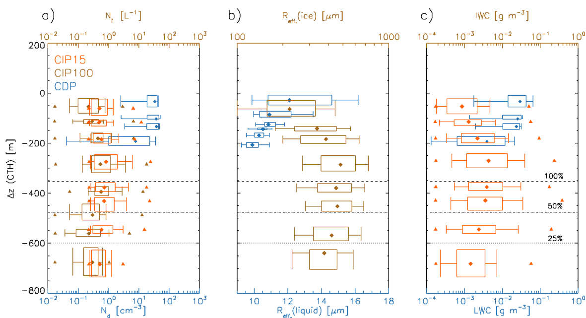
Figure 9. Vertical profiles relative to cloud top of (a) cloud particle number concentrations of liquid, N_d , (CDP [ \text{cm}^{-3} ]) (blue) and ice, N_i , (CIP15 [ \text{L}^{-1} ]) (orange) and (CIP100 [ \text{L}^{-1} ]) (light brown), (b) effective radius for liquid cloud particles, R_{eff}(\text{liquid}) , (CDP) (blue) and ice particles R_{eff}(\text{ice}) , (CIP100) (light brown - upper axis) (c) Condensed water content, CWC, with LWC (CDP) (blue) and IWC (CIP15) (orange). The altitude of observed frequency (areal fraction) of ice-supersaturation is shown for 100 % (black dashed line), 50 % (black dash-dotted line) and 25 % (black dotted line).
