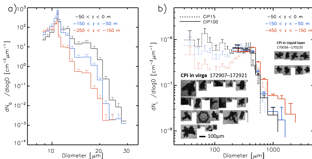
Figure 10. (a) Mean liquid cloud particle size distributions for three vertical levels as Table 3, with cloud top level (black), mid-cloud (blue) and cloud bases (red). Error bars represent standard deviations. (b) Ice particle size distribution from CIP15 (dashed line) and CIP100 (solid line) with colours as (a) and vertical levels as Table 3 with: -50 \text{ m} < z < 0 \text{ m} (black), -150 \text{ m} < z < -50 \text{ m} (blue), -250 \text{ m} (liquid (a)), -450 \text{ m} (ice (b)) < z < -150 \text{ m} (red). Example particle images are taken from CPI probe in ice virga and from within the mixed phase cloud regions, and scale bar is shown for 100 \mu\text{m} length along with the time range of the imagery.
