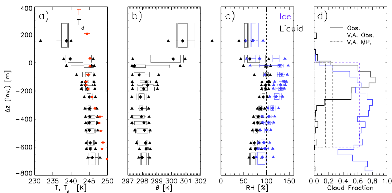
Figure 4. Vertical profiles of statistics w.r.t. inversion altitude, \Delta z_{(inv.)} , for (a) dew point (black), and mean and standard deviation of temperature (red), (b) potential temperature and (c) Relative Humidity w.r.t. Ice (blue) and Liquid (black). Boxes indicate the interquartile range (two-dimensional); bar-and-whiskers: 5 th and 95 th and filled triangles, 1 st and 99 th percentile. (d) Areal cloud fraction calculated from number concentration of liquid (CDP) (black solid) and ice particles (CIP15) (blue solid) over 40 m altitude bins with dashed lines showing the volume mean equivalent fraction over a 600 m deep layer (black - liquid, blue - ice), and calculated mixed-phase cloud fraction in this layer assuming maximum overlap (black dot-dashed line).
