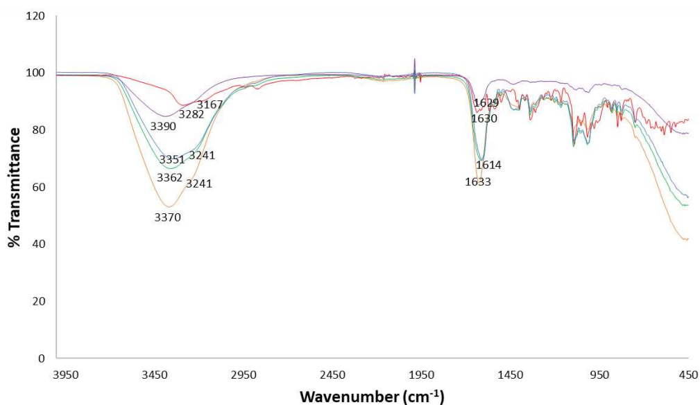
Figure S2. IR spectra of xerogels obtained from DBS-CONH _2 gel (0.4% wt/vol, red line), alginate gel (0.8% wt/vol, purple line) and DBS-CONH _2 /alginate two-component extended interpenetrating gel containing 0.3% wt/vol of DBS-CONH _2 and 0.3% wt/vol alginate (blue line), 0.5% wt/vol alginate (green line) and 1.0% wt/vol alginate (orange line).
