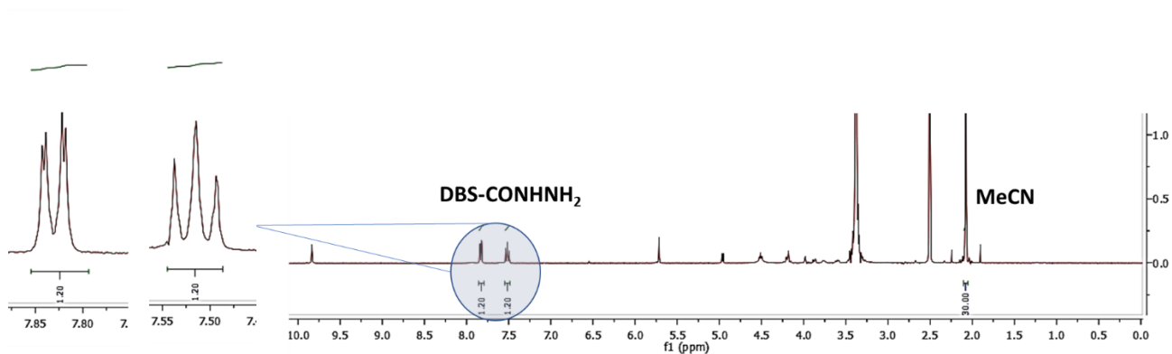
Figure S1. ^1\text{H} NMR of DBS-CONH _2 incorporated into ten DBS-CONH _2 /alginate multicomponent gel beads.
