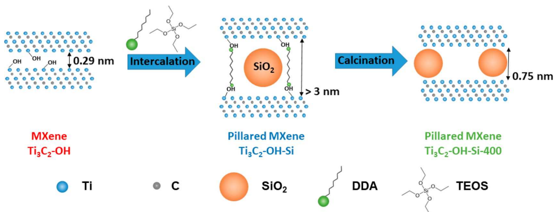
Figure 1. Schematic illustrating the pillaring process of MXenes.
