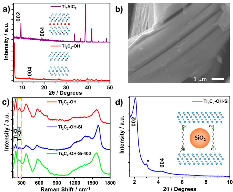
Figure 2. (a) XRD patterns of the as made \text{Ti}_3\text{AlC}_2 , \text{Ti}_3\text{C}_2 after HCl washing ( \text{Ti}_3\text{C}_2\text{-OH} ). The (002) and (004) diffraction peaks were indexed according to Peng et al. 29 (b) SEM micrograph of \text{Ti}_3\text{C}_2 . (c) Raman spectra of the acid treated MXene (red, \text{Ti}_3\text{C}_2\text{-OH} ), and the intercalated (blue, \text{Ti}_3\text{C}_2\text{-OH-Si} ) and calcined at 400 °C (green, \text{Ti}_3\text{C}_2\text{-Si-400} ) pillared MXene, with dashed lines highlighting the key peaks corresponding to Ti-O (gray) and Ti-OH (orange) functional groups. (d) Low angle XRD of the MXene after intercalation ( \text{Ti}_3\text{C}_2\text{-OH-Si} ). The asterisk highlights a peak corresponding to the glass sample holder (see SI Figure S9 for sample holder reference spectra).
