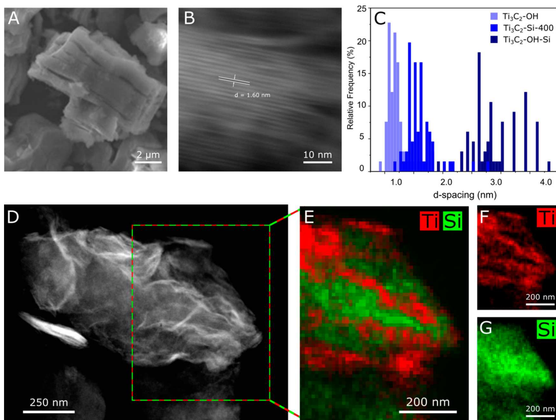
Figure 3. SEM and STEM Characterization of the pillared MXene. (a) SEM micrograph of the intercalated MXene ( \text{Ti}_3\text{C}_2\text{-OH-Si} ). (b) STEM cross sectional image of atomic planes of \text{Ti}_3\text{C}_2\text{-OH-Si-400} , with an example d -spacing labeled. (c) Graph showing the results of the 002 interlayer distances measured using STEM. (d–g) STEM-EDS mapping of the pillared sample post calcination ( \text{Ti}_3\text{C}_2\text{-OH-Si-400} ).
