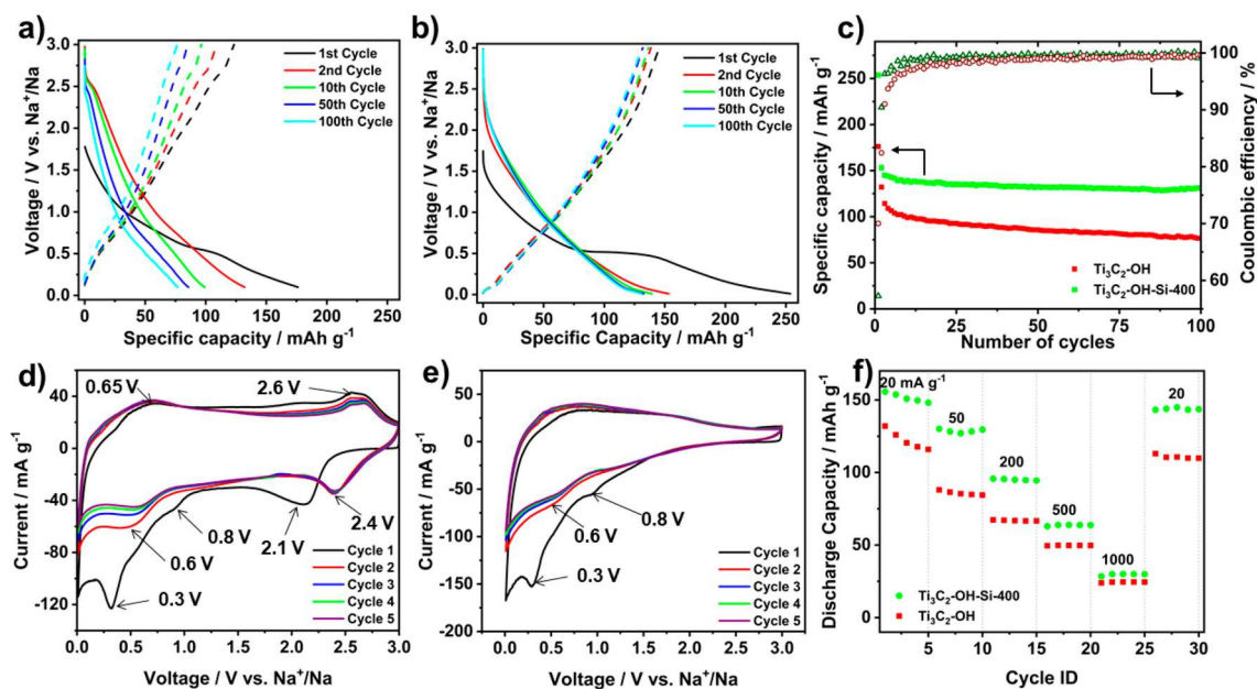
Figure 7. Galvanostatic data from half-cell tests against Na metal at 20 \text{ mA g}^{-1} in the voltage range 0.01–3 V. Load curves for selected cycles for (a) \text{Ti}_3\text{C}_2\text{-OH} and (b) \text{Ti}_3\text{C}_2\text{-OH-Si-400} . (c) Coulombic efficiency and discharge capacities of the pillared and nonpillared samples over 100 cycles. Cyclic voltammograms at 0.01–3 V vs Na metal at a scan rate of 0.2 \text{ mV s}^{-1} for (d) the nonpillared, \text{Ti}_3\text{C}_2\text{-OH} and (e) pillared MXene, \text{Ti}_3\text{C}_2\text{-OH-Si-400} . (f) Rate capability tests for the pillared and nonpillared MXene at rates of 20, 50, 200, 500, and 1,000 \text{ mA g}^{-1} . Five cycles are shown for each rate (one additional cycle at 20 \text{ mA g}^{-1} was conducted to ensure SEI formation).
