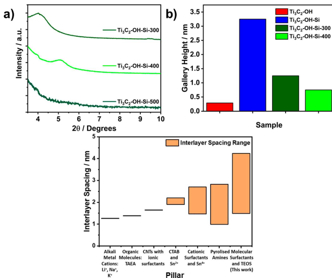
Figure 4. Effect of calcination temperature on interlayer spacing and gallery height. (a) XRD patterns tracking the (002) diffraction peak after different calcination temperatures (300, 400, and 500 °C). (b) Chart showing the range of gallery heights achieved using the reported pillaring method. (c) Comparison of interlayer spacings achieved in this work with other pillaring reports.
