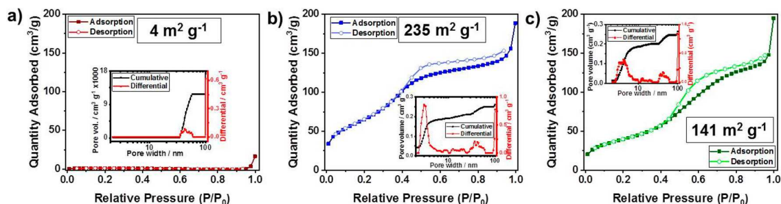
Figure 5. Adsorption isotherms from N_2 adsorption–desorption experiments. The BET surface area is also given in each panel. (a) Ti_3C_2-OH , (b) Ti_3C_2-OH-Si , and (c) Ti_3C_2-OH-Si-400 . Insets: Pore size distributions derived from the NL DFT method for each sample.
