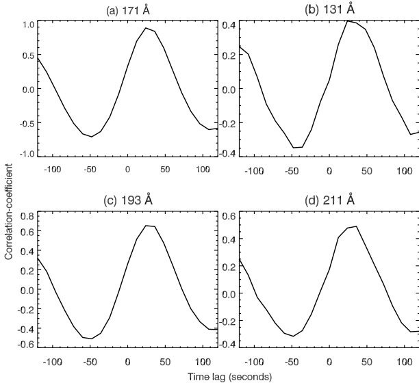
Fig. 7. Cross-correlation analysis performed between detrended light curves obtained from locations L1 and L2 of the time-distance maps (locations shown by yellow dashed lines in Figs. 4 and 5). The cross-correlation coefficient is plotted on the y-axis as a function of time lag in seconds on the x-axis.
