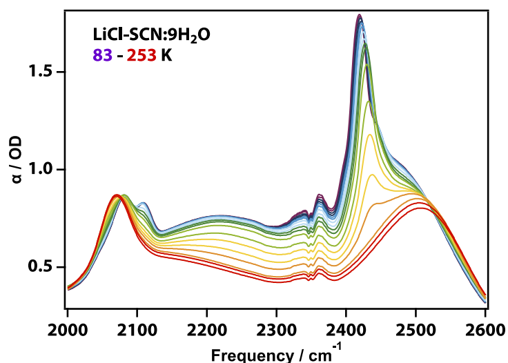
Figure. 2. IR spectra of the non-eutectic LiCl-SCN:9H 2 O solution doped with D 2 O measured from 83 to 253 K. Raw spectrum showing the \nu_{CN} asymmetric stretch ( \sim 2080 \text{cm}^{-1} ), H 2 O combination band of the H-O-H bend and librational mode ( \delta_{HOH}+\nu_{lib} , \sim 2200 \text{cm}^{-1} ), and the \nu_{OD} stretching mode of ice (2430 \text{cm}^{-1} ) and the \nu_{OD} mode of liquid water ( \sim 2500 \text{cm}^{-1} ).
