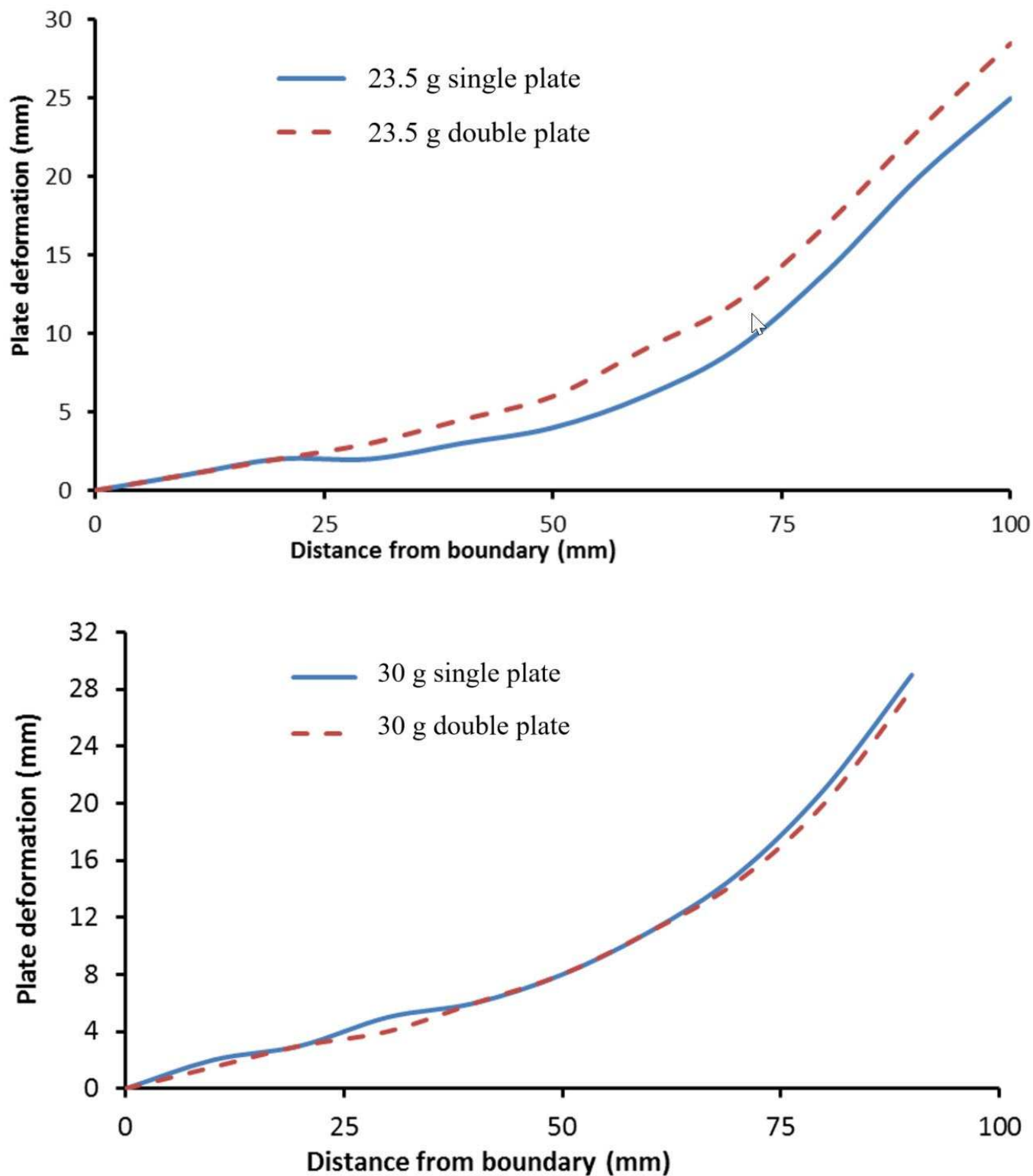
Figure 7: Deformation profiles of single and double (front) plates subjected to (a) 23.5 g detonations (b) 30 g detonations
