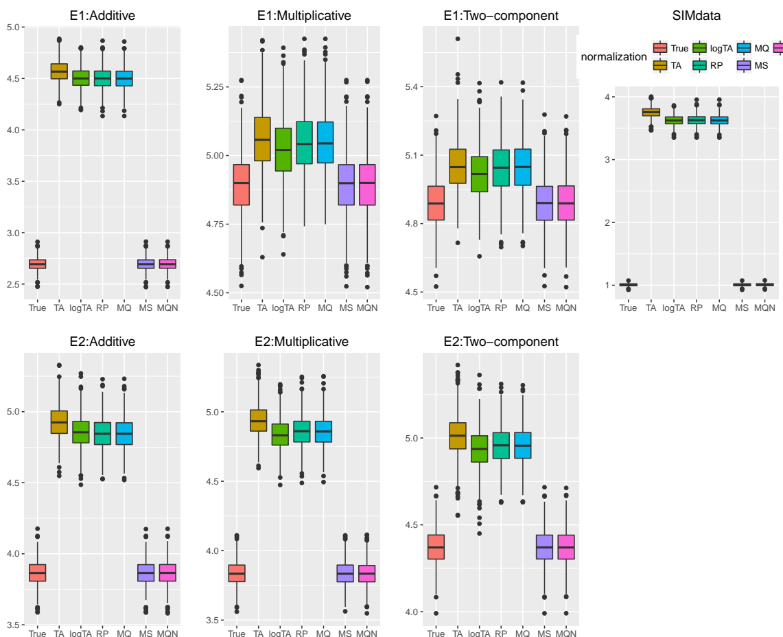
Figure 5: Comparison of prediction performance based on prediction error; the smaller error, the better performance. SIMdata in the right shows the prediction error without introducing error. (i) Under the error model E1: In the case of perturbation of additive error, the column-wise normalized (MS and MQN) data performed similarly well. When multiplicative error is present (multiplicative or two-components), multiplicative error dominates. (ii) The lower row shows the error model E2, which has smaller multiplicative error than E1. The results show similar prediction error patterns as in (i). Throughout all scenarios, the column-wise normalization methods outperform the row-wise ones; i.e., smaller prediction error using MS and MQN.
