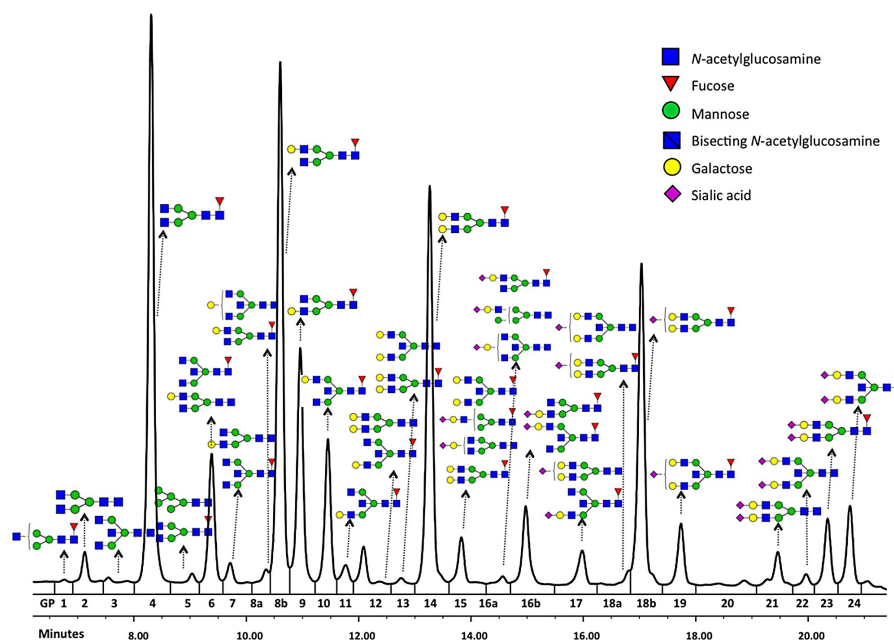
Figure 1: Typical chromatogram of glycans separated by HILIC-UPLC analysis of the IgG glycome. Raw glycan intensities are computed as areas under the curve of corresponding chromatographic peak (GP1-24).
