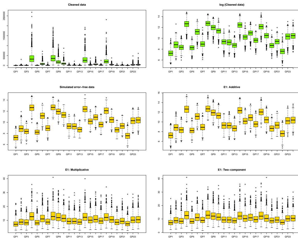
Figure 4: Distribution of glycans with correlated error. The green and yellow color depicts the measured and simulated data, respectively. (i) The first row, colored green, depicts the cleaned and its log-transformed data: the extreme range of abundance and the highly right skewed distribution of cleaned data can be dealt with the log-transformation of the data. (ii) The second row shows error-free simulated data based on the log-transformed cleaned data, and the error-contaminated data with additive error (E1), which showed similar distribution patterns. (iii) The last row multiplicative and two-component error under E1. Introducing multiplicative error in glycans made the distribution skewed, and the range of abundances larger. The similarity of two distribution patterns indicates that multiplicative error dominates additive error.
