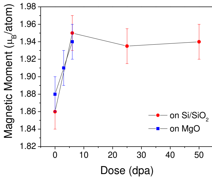
Fig.5. The magnetic moment versus dose for Fe-10at%Cr determined by least squares fit to the reflectivity data (see for example Fig. 4).
