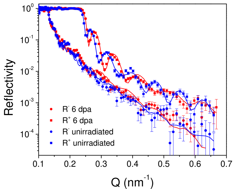
Fig.4. PNR spectra for the unirradiated and the 6 dpa irradiated Fe-10at%Cr alloy. The solid lines are least squares fits to the data.
