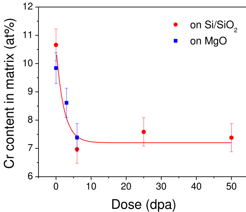
Fig.6. The Cr content in the FeCr matrix versus dose, for the Fe-10at%Cr alloy, as calculated from the magnetic moments of Fig. 5 and eq. (5). The continuous line is a least squares fit to the data (eq. (7)).
