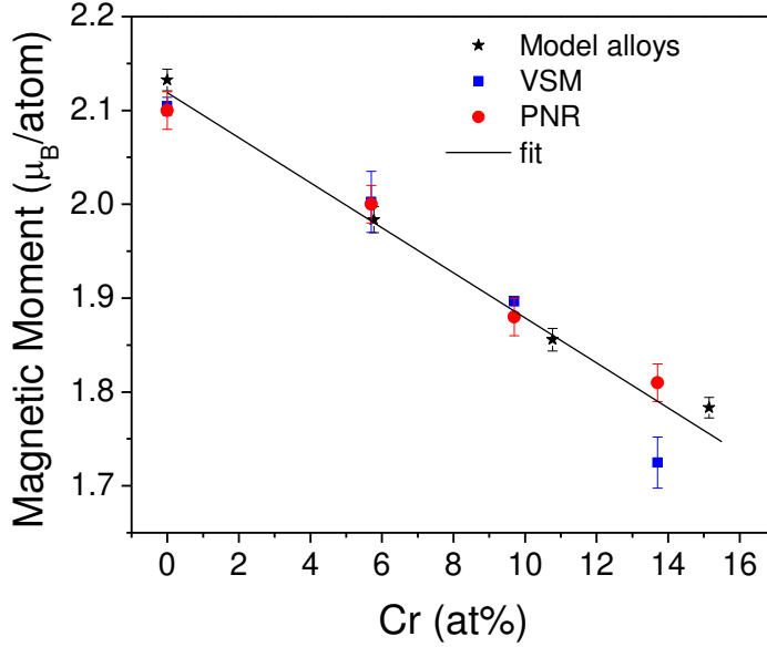
Fig.2. The magnetic moment per atom of the as-fabricated samples as a function of Cr content determined by both PNR and VSM measurements and the magnetic moment of FeCr bulk alloys [44] as determined by VSM. The solid line is a least squares fit to all the data.
