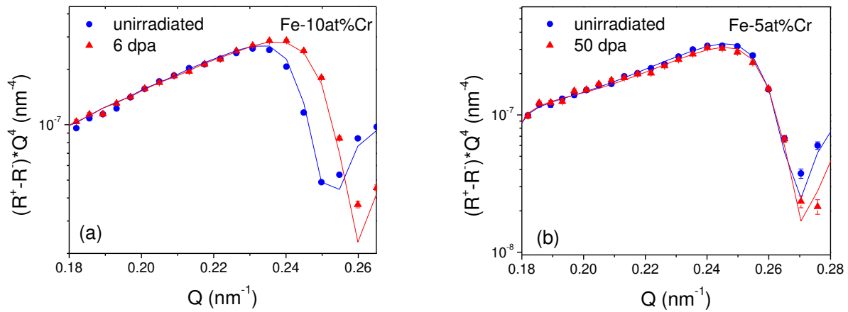
Fig.3. Spin asymmetry (R^+ - R^-)Q^4 at the critical edge. The solid lines are least squares fits to the data. 3(a): Fe-10at%Cr alloy unirradiated and irradiated at 6 dpa. 3(b): Fe-5at%Cr alloy unirradiated and irradiated at 50 dpa.
