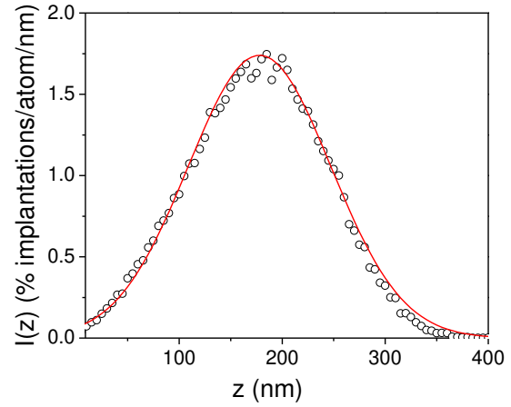
Fig. 1b. Percentage of implanted Fe ions over the number of atoms in the sample as a function of depth of Fe-10at%Cr films irradiated by 490 keV Fe + ions, computed by SRIM for 50 dpa and a flux of 1.8 \times 10^{12} ions/(cm 2 ·s). Solid line: see text for details.
