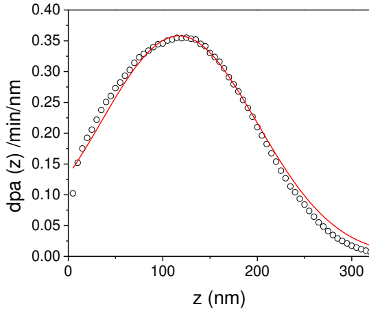
Fig. 1a. Damage rate as a function of depth of Fe-10at%Cr films irradiated by 490 keV Fe + ions, computed by SRIM for a flux of 1.8 \times 10^{12} ions/(cm 2 ·s). Solid line: see text for details.
