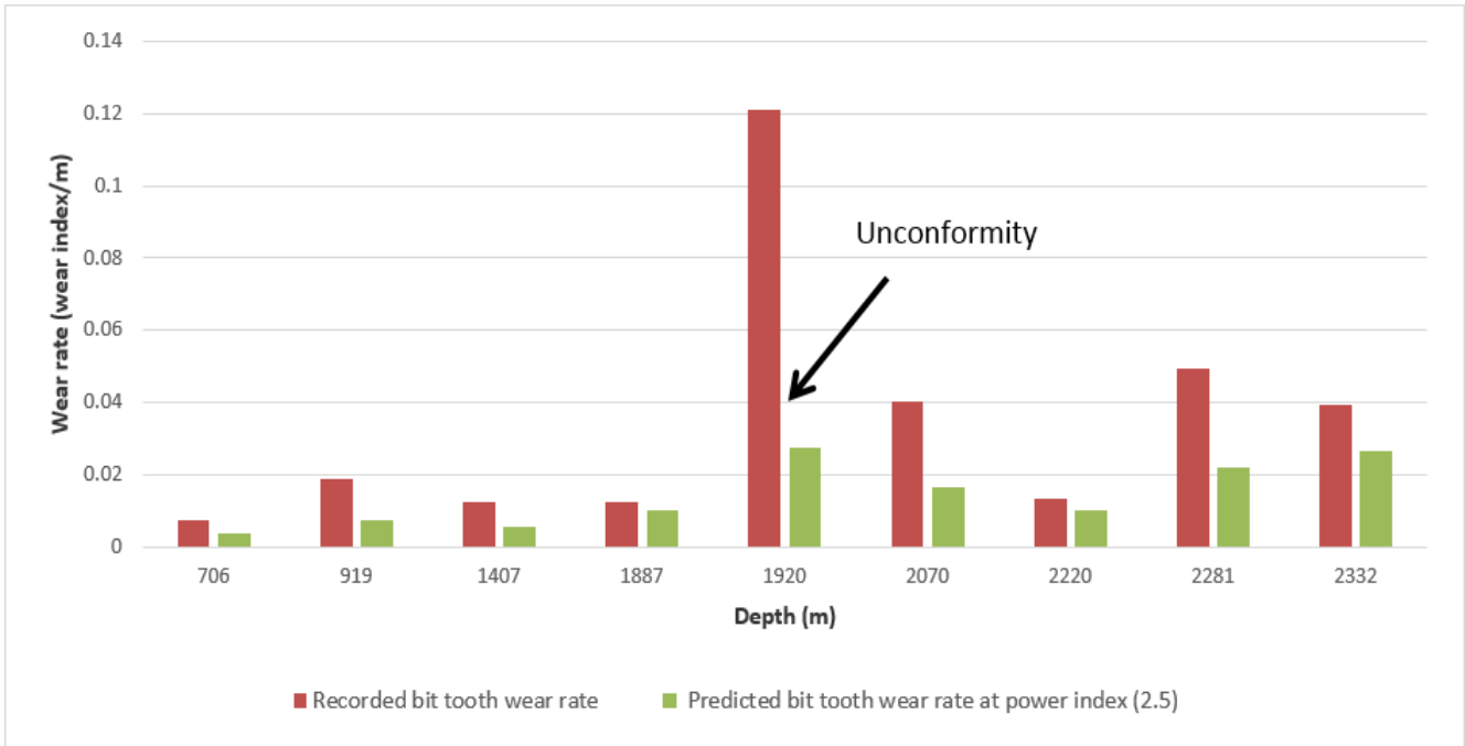
Figure (10) Anticipated bit tooth dullness rate compared with the in-situ qualitative bit insert dullness rate for well A 2 in south of Iraq
