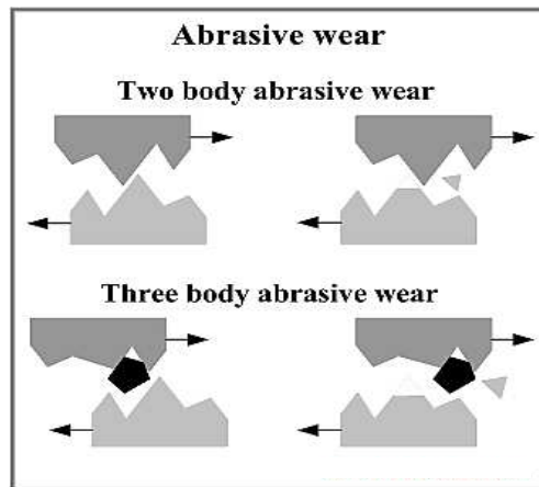
Figure (3) Comparison between (a) two-body abrasion and (b) three-body abrasive wear (Reprinted from Ref [22])
