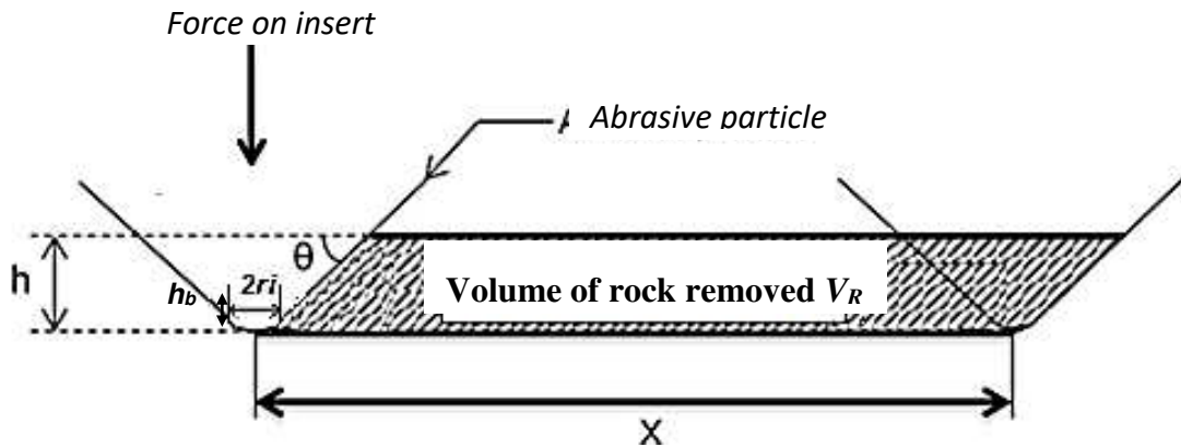
Figure (4) Modified model of bit tooth dullness (based on Rabinowicz [15])
