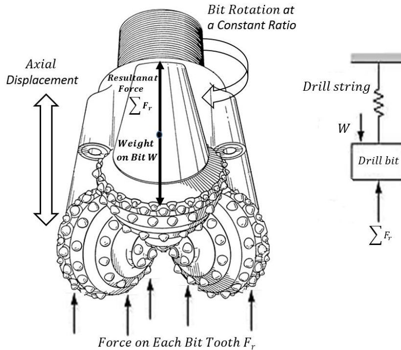
Figure (5) Forces affecting the tri-cone drill bit and the cutters [26,28]
