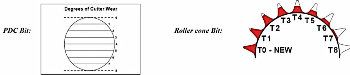
Figure (1) Wear grading system for bit tooth (insert) [12]
