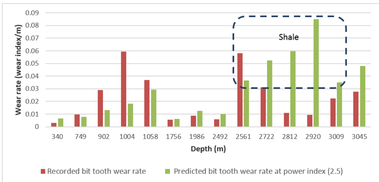
Figure (9) Anticipated real-time insert dullness rate obtained from exponent index 2.5 compared to the in-situ qualitative bit insert dullness rate for well B 2
