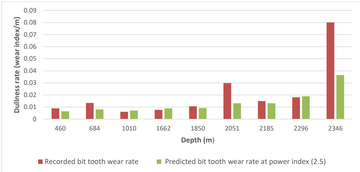
Figure (8) Anticipated dullness rate obtained from exponent index 2.5 compared with in-situ qualitative bit tooth dullness rate for well B 1
