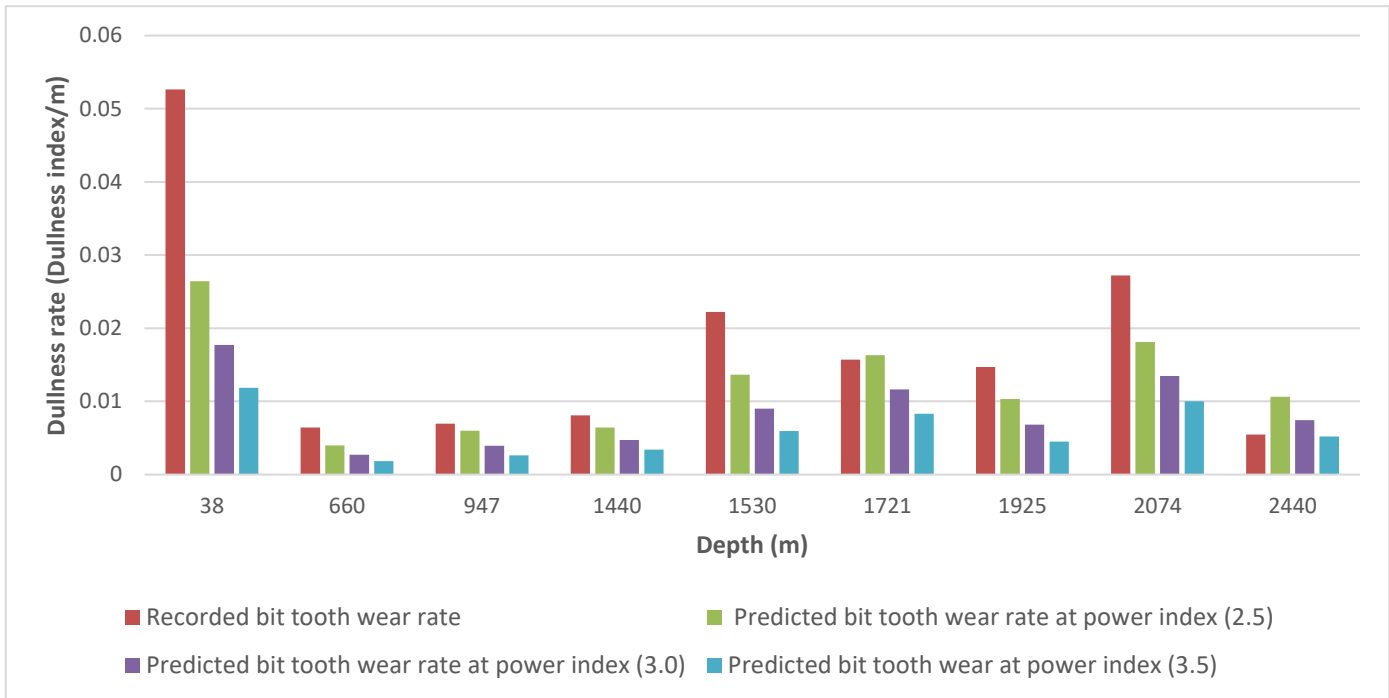
Figure (7) Real-time anticipated tooth dullness (wear) rate of various powers of equation (20) along with the real-time field bit tooth dullness rate for well A 1 in Basrah region South of Iraq
