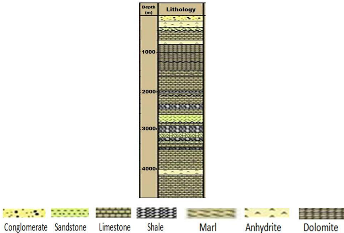
Figure (2) Lithological stratigraphic of rock formation in Basrah, Southern Iraq [20].
