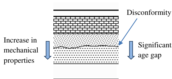
Figure (11) Development of disconformity [31]
