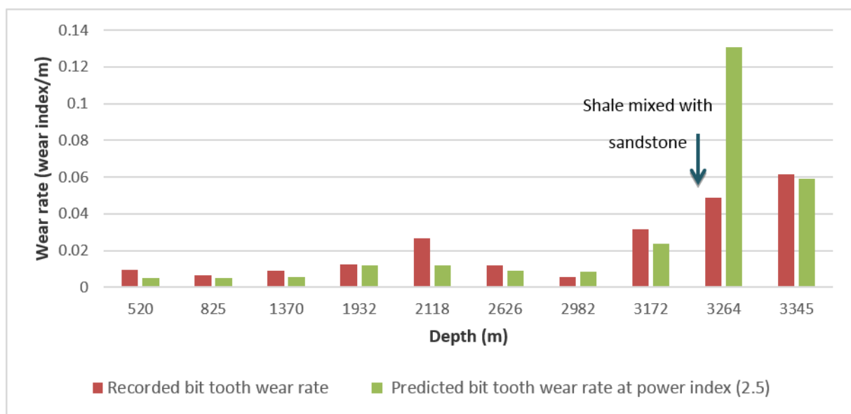
Figure (12) Real-time anticipated dullness rate compared with the real-time in-situ qualitative bit tooth dullness rate for well B 3
