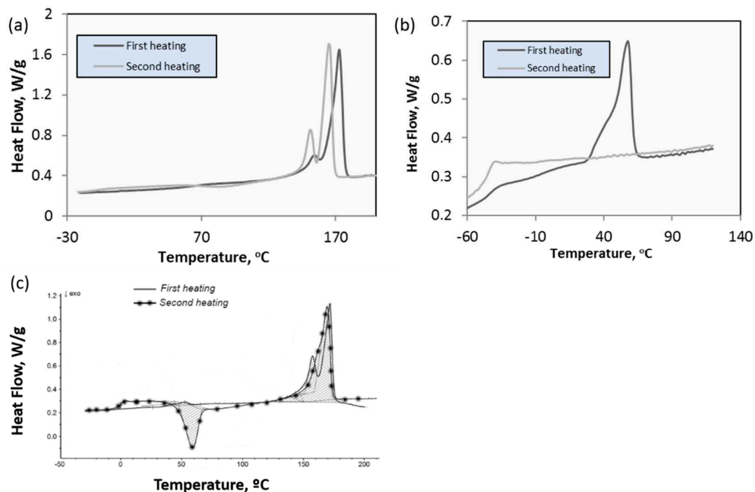
Figure 14. DSC curves of scl- (a) and mcl- (b) PHAs and the blend (c).
