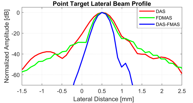
Fig. 2. Lateral beam profiles of the wire target at the depth of 30 mm when using beamforming techniques DAS, FDMAS and DAS-FMAS.
