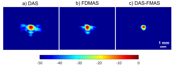
Fig. 1. B-mode images of the wire target beamformed using a) DAS, b) FDMAS and c) DAS-FMAS with 25 plane waves.
