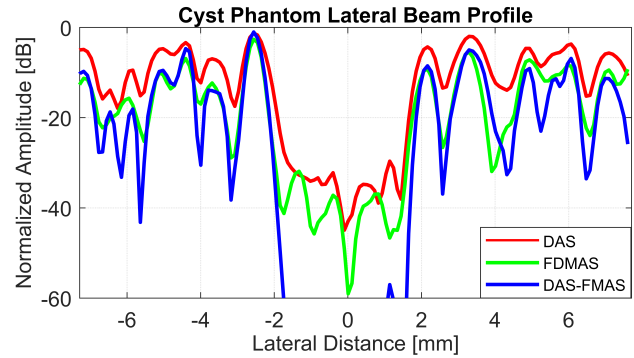
Fig. 5. Beam profiles for DAS, FDMAS and DAS-FMAS along the lateral direction at the 15 mm depth for the cyst of 3 mm in diameter.
