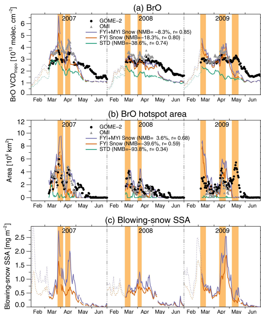
Figure 4. Time series of daily mean BrO VCD_{\text{tropo}} , tropospheric BrO hotspots area, and blowing-snow SSA burden over high latitudes ( > 60^\circ \text{N} ) between February and June for 2007–2009. (a) Time series of daily VCD_{\text{tropo}} (in 10^{13} molecules \text{cm}^{-2} ) averaged poleward of 60^\circ \text{N} for GOME-2 (black circles) and OMI (gray triangles) and simulated with GEOS-Chem (FYI+MYI Snow, purple; FYI Snow, orange; and STD, green). (b) The daily area extent of BrO hotspots (in units of 10^6 \text{km}^2 ) for GOME-2, OMI, and GEOS-Chem. See Sect. 3.3 for the definition of BrO hotspot areas. Note that the total area poleward of 60^\circ \text{N} is 34.2 \times 10^6 \text{km}^2 . (c) Time series of the daily mean blowing-snow SSA burden ( \text{mg m}^{-2} ) for the FYI+MYI Snow and FYI Snow simulations. The blowing-snow SSA burden is obtained as the difference between the blowing-snow and STD simulations. The normalized mean bias (NMB) and Pearson correlation coefficients displayed in panels (a) and (b) are relative to the combined GOME-2 and OMI time series. The events highlighted in light orange are defined as periods when GOME-2 or OMI BrO hotspots cover more than 2 \times 10^6 \text{km}^2 for longer than 5 d. We only show days where valid satellite observations are available over at least 70 % of the surface area poleward of 60^\circ \text{N} . The dashed lines in panels (a) and (c) correspond to the GEOS-Chem daily means poleward of 60^\circ \text{N} for days with less than 70 % of valid observations.
