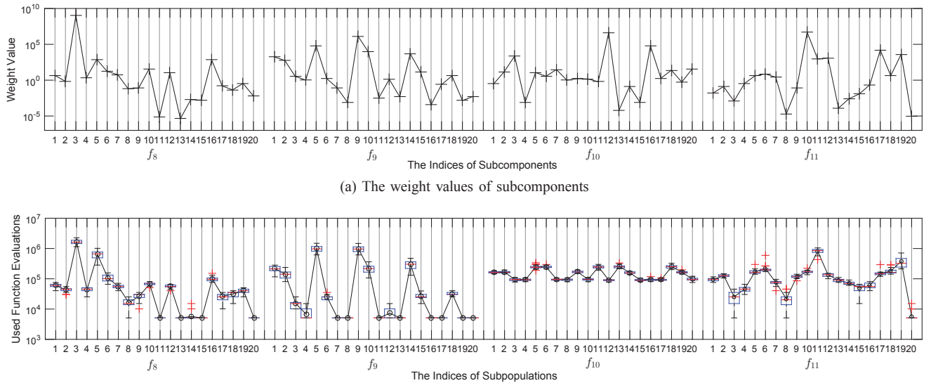
(b) The box plot of the function evaluations used by each subpopulation to optimize its corresponding subcomponent over 25 independent runs, where the circle point show the mean number of function evaluations used by each subpopulation over 25 independent runs.
