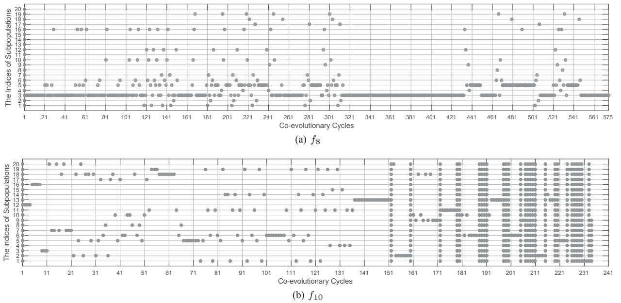
Fig. 2. The activation of subpopulations in a run on two selected CEC'2013 functions for CCFR-I, where the filled circle point denotes that the subpopulation undergoes evolution in the corresponding co-evolutionary cycle.
