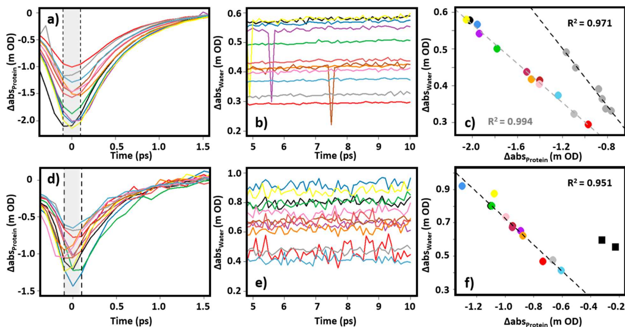
Figure 2. (a–c) Vibrational relaxation dynamics obtained from IR pump–probe spectroscopy (LIFETIME instrument) of 50 mg/mL BSA in \text{H}_2\text{O} buffer. (a) Temporal dynamics of the amide I response at 1653\text{ cm}^{-1} at pump–probe delay times <1.5 ps. (b) Water response at 1634\text{ cm}^{-1} at pump–probe delay times from 5 to 10 ps. (c) Linear correlation arising from plotting the water signal averaged between pump–probe delay times of 5–10 ps against the average protein absorbance from pump–probe delay times of \pm 0.1 ps (shaded area in part a). Results for a BSA concentration of 50 mg/mL are shown as colored circles. Data for 30 mg/mL BSA samples are shown using gray circles. Parts d–f show similar data to that in parts a–c but obtained using the ULTRA instrument and 30 mg/mL BSA in \text{H}_2\text{O} buffer. (d) Temporal dynamics of the amide I response at 1656\text{ cm}^{-1} at pump–probe delay times <1.5 ps. (e) Water response at 1634\text{ cm}^{-1} at pump–probe delay times from 5 to 10 ps. (f) Linear correlation arising from plotting the water signal averaged between 5 and 10 ps against the average protein absorbance from \pm 0.1 ps (shaded area in part d). In all cases, each data point indicates a different measurement of the same stock solution. Dashed lines indicate linear fits to the data. The black squares in part f indicate results obtained from pure water samples for comparison (see text).
