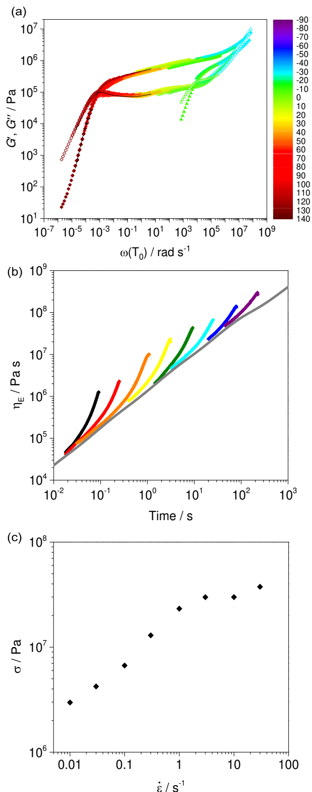
Fig. 5 (a) Rheology master curves for UPy1 ( \Delta ) and Am1 ( \heptagon ) shifted using WLF theory. G' solid symbols, G'' open symbols. Colour scale corresponds to the temperature of measurement, in degrees celcius. Maxwell mode fit shown with black lines.. T_0=25 °C (b) Extensional (open symbols) viscosity of UPy1, at 25 °C, at strain rates of: 30 ( \blacklozenge ), 10 ( \blacklozenge ), 3 ( \blacklozenge ), 1 ( \blacklozenge ), 0.3 ( \blacklozenge ), 0.1 ( \blacklozenge ), 0.03 ( \blacklozenge ) and 0.01 ( \blacklozenge ) s^{-1} . Linear prediction of viscosity ( \blacklozenge ). (c) Maximum extensional stress of UPy1 before sample fracture.
