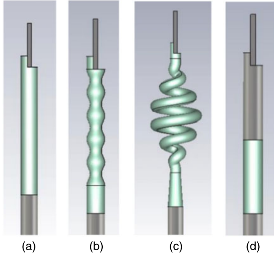
Figure 11. Side elevation of stalk designs used in 3D PIC simulations. Transparent grey sections represent a perfect electrical conductor (PEC), while the grey-green regions represent Teflon plastic. (a) Standard cylindrical stalk configuration: pure Teflon and PEC models were used. (b) Sinusoidally modulated Teflon stalk. (c) Teflon spiral stalk. (d) Half-length Teflon and PEC stalk.
