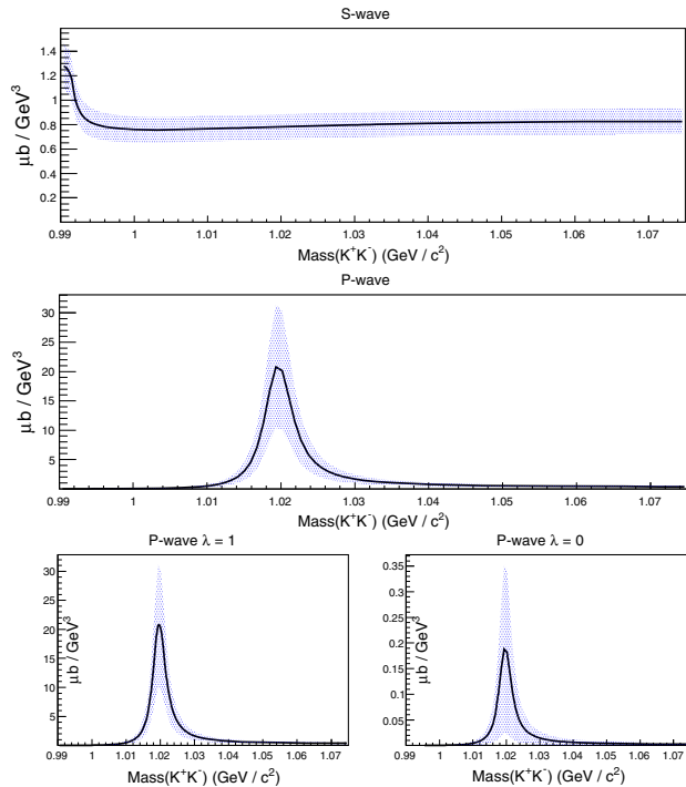
FIG. 14. Magnitudes of the S and P partial waves along with two-spin projections of the P wave ( \lambda_{KK} = 1, 0 ) in the 0.7 \leq t \leq 0.8 \text{ GeV}^2 bin determined by fitting to the experimental moments.
