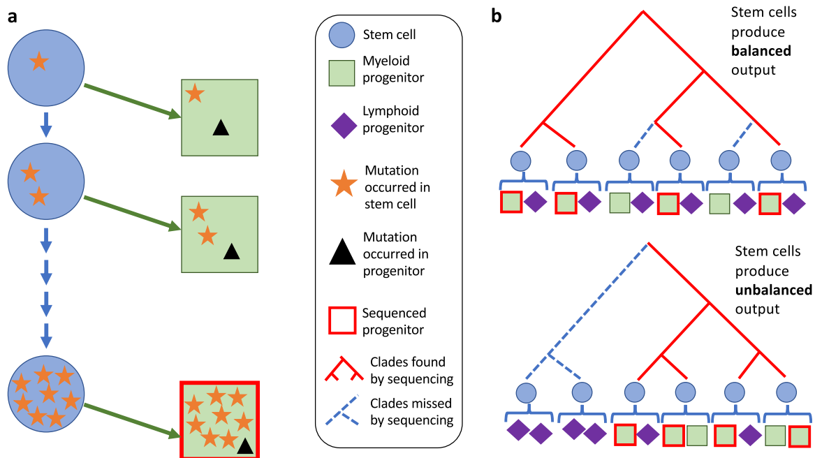
Figure 2. Effect of cell types that are sequenced on studies. (A) Sequencing progenitors reveals mutations that occurred in stem cells. Mutations that occurred in stem cells accumulate over time. When a progenitor from an adult is sequenced, most of the mutations discovered occurred in stem cells. (B) The cell types that are sequenced may affect the phylogeny that is reconstructed if stem cells do not produce balanced output. In the top phylogeny, all stem cells produce both myeloid and lymphoid cells. Sequencing only myeloid progenitors samples the phylogeny evenly, such that an accurate representation of the phylogeny is reconstructed. In the bottom phylogeny, some stem cells produce disproportionately more lymphoid than myeloid progenitors. Sequencing only myeloid progenitors undersamples parts of the phylogeny that are biased toward lymphoid cells.
