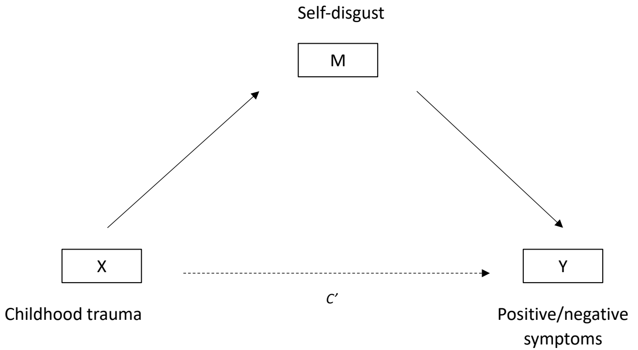
Figure 1. Path diagram of unadjusted mediation model testing if self-disgust mediates the relationship between childhood trauma and symptoms of psychosis. N.B. positive and negative symptoms will be tested in separate models but are included in the same diagram here for illustrative purposes.
