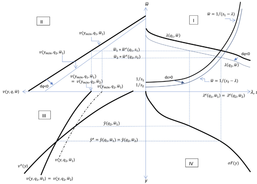
Fig. 2. Effect of ( dq < 0 , ds > 0 ) which keep equilibrium expected demand \lambda^e(q, s) constant. Initial equilibrium at q_1, s_1 has expected waiting time \bar{w}_1 = \bar{w}^e(q_1, s_1) , equilibrium expected demand \lambda^e(q_1, s_1) . New equilibrium at q_2 = q_1 + dq < q_1 , s_2 = s_1 + ds > s_1 has expected waiting time \bar{w}_2 = \bar{w}^e(q_2, s_2) < \bar{w}_1 = \bar{w}^e(q_1, s_1) , equilibrium expected demand \lambda^e(q_2, s_2) = \lambda^e(q_1, s_1) . v(y, q, \bar{w}) and v^o(y) are expected utility for individuals who chose the public hospital and the outside option of private treatment when ill, respectively. \hat{y}(q, \bar{w}) critical income of marginal public hospital patient.
