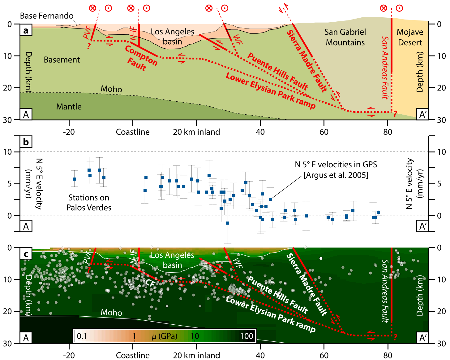
Figure 2. (a) Cross sections of faults, structure, north-south contraction, and seismicity along profile A-A'. Red lines are fault surfaces as meshed here (Figure 3), dashed where uncertain (Shaw & Suppe, 1996; Shaw & Shearer, 1999; Fuis et al., 2012). Geometries of basin, basement, and mantle are from Shaw et al. (2015); geometry of base of Fernando Formation (boundary between beige and tan units of the basin) is interpolated from Sorlien et al. (2013; offshore), Wright (1991; coastline to Whittier Fault), and Yeats (2004; Whittier Fault to Sierra Madre Fault); topography is from Fuis et al. (2012). (b) Projections of Argus et al. (2005) GPS velocities (relative to San Gabriel Mountains) onto the direction N 5° E and 1σ uncertainties. Note that stations on Palos Verdes are plotted left of the coastline as the offshore section of profile A-A' passes alongside Palos Verdes (Figure 1a). (c) Seismotectonic features. Distribution of shear modulus is from the CVM*, the heterogeneous elastic model used in this study (section 4). Translucent white circles are relocated 1981–2016 M \geq 2 earthquakes whose epicenters lie within the mesh area of the three thrust faults and decollement (Hauksson et al., 2012 and updated). PVF = Palos Verdes Fault; N-IF = Newport-Inglewood Fault; WF = Whittier Fault.
