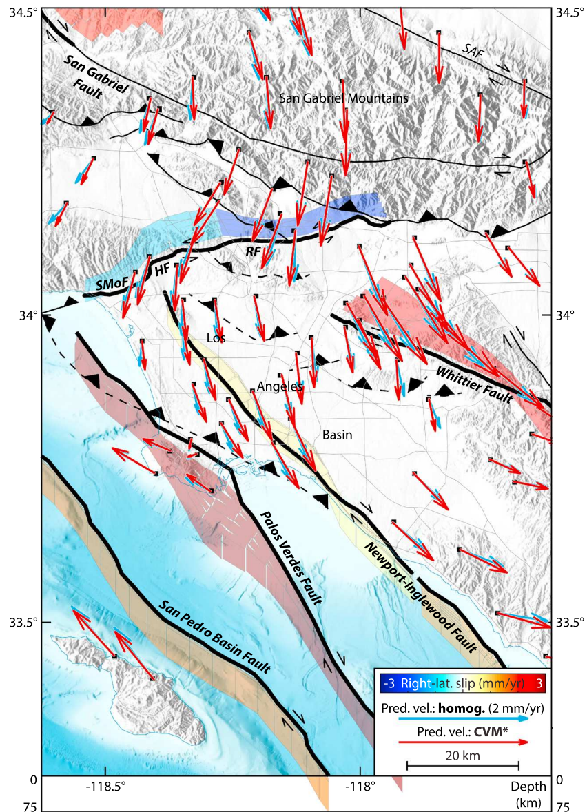
Figure 5. Strain accumulation on local strike-slip faults could contribute up to \sim 1.8 mm/year of north-south shortening, as shown here with a forward model in which the strike-slip faults slip at their UCERF3 consensus “Geologic” slip rates between \sim 5 - and 75-km depths. Blue and red arrows are the predicted surface velocity fields calculated in a homogeneous half-space and in the CVM*, respectively. (Look angle is slightly northward rather than vertically down; San Pedro Basin Fault, Palos Verdes Fault and southern Newport-Inglewood Fault all dip vertically.) SAF = San Andreas Fault; SMoF = Santa Monica Fault; HF = Hollywood Fault. RF = Raymond Fault.
