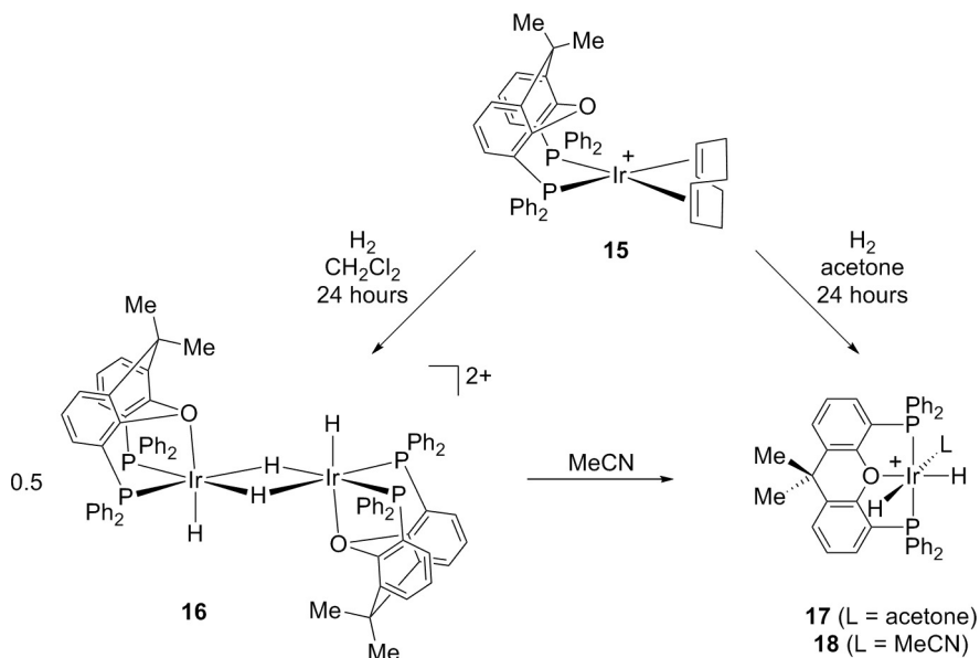
Scheme 8. Weller's cationic \{\text{Ir}(\text{Xantphos-Ph})\} complexes which show differing coordination modes depending on the conditions. \text{BAR}_4^{\ominus} anions omitted for clarity.
