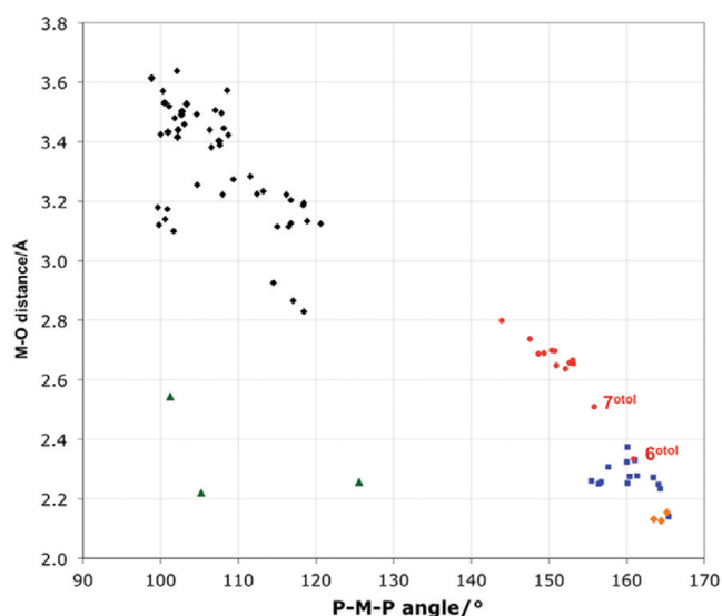
Fig. 3. Plot of M–O distance (Å) versus P–M–P bond angle ( ^\circ ) of \{M(\text{Xantphos-Ph})\} complexes by Haynes and co-workers (M = transition metal). Reprinted with permission from G.L. Williams, C.M. Parks, C.R. Smith, H. Adams, A. Haynes, A.J.H. M. Meijer, G.J. Sunley, S. Gaemers, Organometallics 30 (2011) 6166–6179. Copyright 2011 American Chemical Society.
