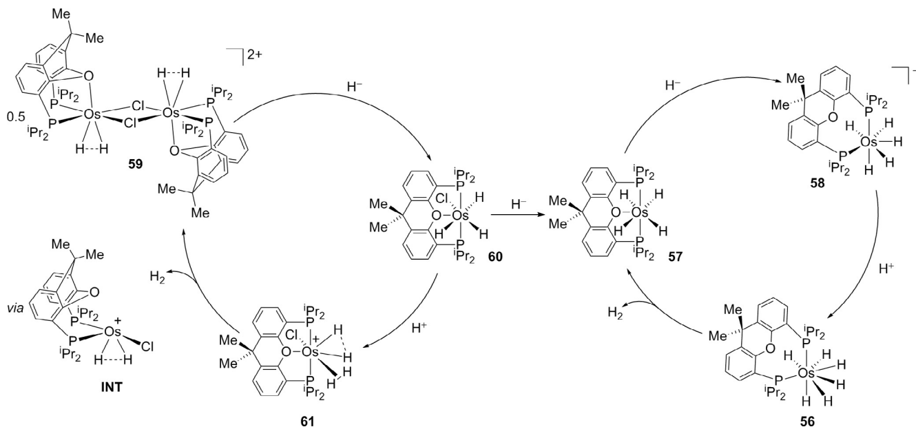
Scheme 20. Variable coordination modes of the Xantphos- 1 Pr ligand.
