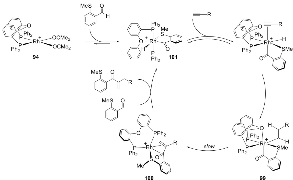
Scheme 29. Proposed catalytic cycle for the hydroacylation of alkynes to form the branched alkenyl product using the {Rh(DPEphos)} + fragment. CB 11 H 12 anion omitted for clarity.
