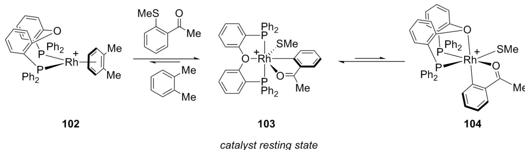
Scheme 30. fac-mer isomerisation of the catalyst resting state during the carbothiolation of alkynes using a {Rh(DPEphos)} + fragment. BAR 4 + anions omitted for clarity.
