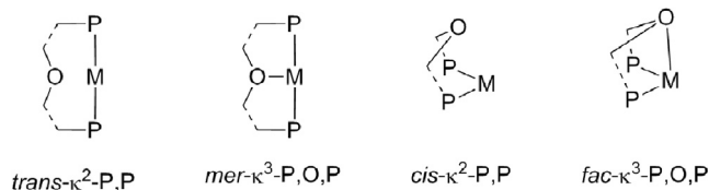
Fig. 2. Ligand flexibility and hemilability in POP-type ligands.
