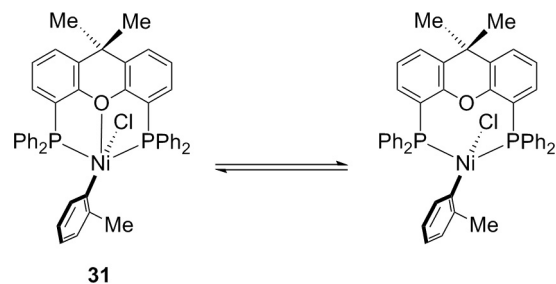
Scheme 12. The postulated hemilabile nature of the Xantphos-Ph ether linker in trans -Ni( o -C 6 H 4 (CH 3 ))(Cl)( \kappa^3 -P,O,P-Xantphos-Ph).
