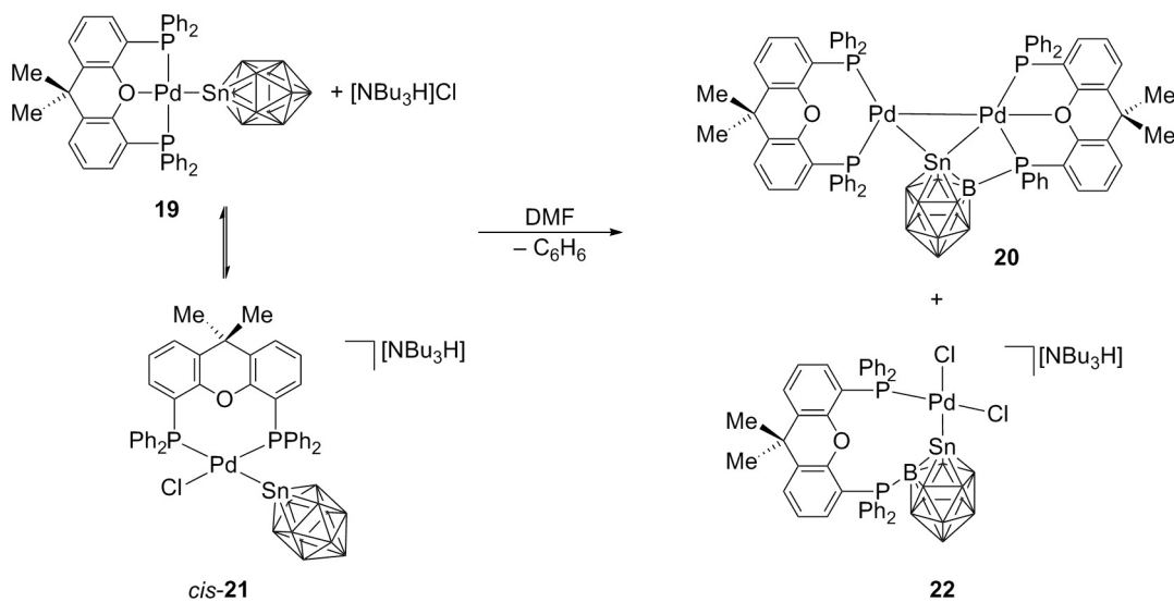
Scheme 9. Palladium complexes of stanna- closo -dodecaborate, showed \kappa^3 -P,O,P, \kappa^2 -P,P and \kappa^1 -P-bound Xantphos-Ph, and the equilibrium between the \kappa^3 -P,O,P and \kappa^2 -P,P-complexes 19 and 21 . Unlabelled vertex = B-H.
