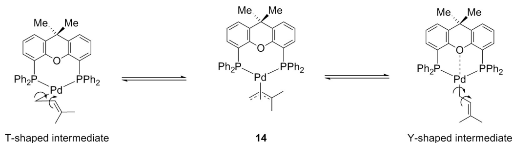
Scheme 7. Proposed intermediates for the \pi - \sigma rearrangement in \text{Pd}(\eta^3\text{-}1,1\text{-}(\text{CH}_3)_2\text{C}_3\text{H}_3)(\kappa^2\text{-P,P-Xantphos-Ph}) .
