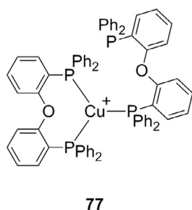
Fig. 6. Structure of [Cu(DPEphos) 2 ] + showing the tricoordinate Cu(I) centre. BF 4 - anion omitted for clarity.
