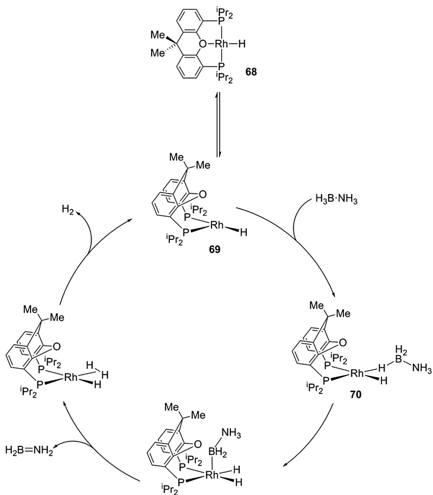
Scheme 22. Calculated catalytic cycles for the dehydrogenation of ammonia borane using mer - \kappa^3 -P,O,P-Xantphos- i Pr complex 68 .
