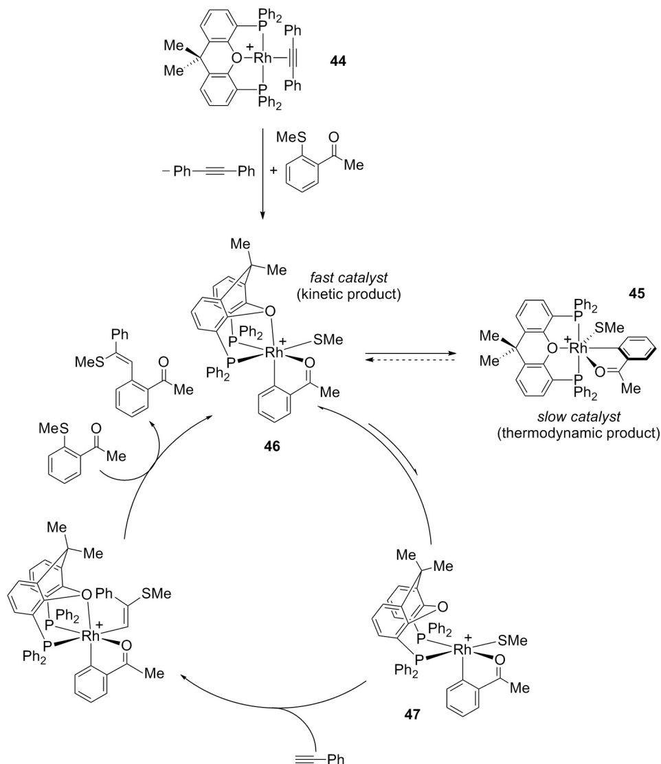
Scheme 17. Proposed catalytic cycle for the catalytic carbothiolation of phenylacetylene using the \kappa^3 -P,O,P-Xantphos-Ph catalyst 44 , mer -[Rh(PhCCPh)( \kappa^3 -P,O,P-Xantphos-Ph)][BAR 4 F ]. BAR 4 F anions omitted for clarity.
