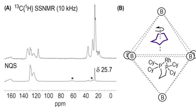
Figure 4. (A) ^{13}\text{C}\{^1\text{H}\} SSNMR spectra (10 kHz, 158 K) and NQS spectra of [2][\text{COACBAR}^{\text{F}}_4] (10 kHz, 158 K). * = spinning sideband. (B) Proposed fluxional processes (B = [\text{BAR}^{\text{F}}_4] ).
