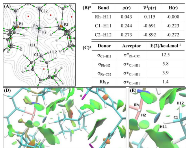
Figure 13. (A) Molecular graph of the [4\text{-COA}]^+ cation; density contours plotted in the RhH11C1 plane, BCPs (green), and RCPs (red). (B) Key BCP metrics and (C) donor–acceptor interactions associated with the Rh–H11C1 interaction. (D) NCI plot of the [4\text{-COA}][\text{BAR}^{\text{F}}_4] ion pair; isosurface generated for s = 0.3 au and -0.07 < \rho < 0.07 au. (E) Detail highlighting the region around Rh.
