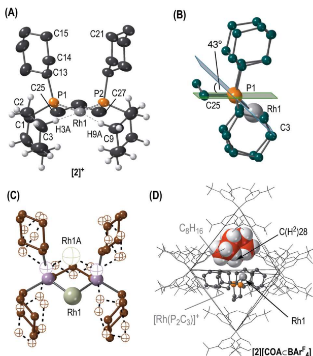
Figure 3. (A) Cation of [2][\text{COACBAR}^F_4]^+ . 50% displacement ellipsoids, only the major disordered component shown. Selected bond lengths (Å) and angles (deg): Rh1...C3, 2.912(10); Rh1...C9, 2.873(10); Rh1-P1, 2.171(2); Rh1-P2, 2.166(2); P1-Rh1-P2, 91.21(8); \angle \text{P1P2C25C27/Rh1P1P2} , 42.6(2). (B) Displacement of the Rh center in [2]^+ toward the agostic C-H bonds in the major disordered component. (C) Ball and stick representation of the two disordered components in [2]^+ . (D) Packing diagram of [2][\text{COACBAR}^F_4] showing the O_h arrangement of [\text{BAR}^F_4]^- , COA (C = red) shown at van der Waals radii, and only one disordered component shown, Rh1...C28, 3.74(1) Å.
