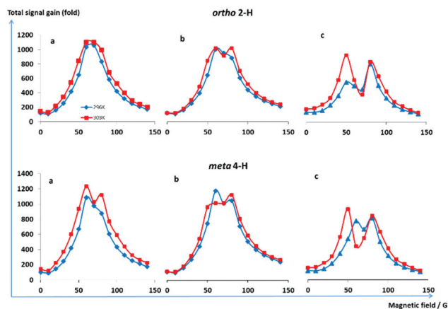
Fig. 2 (a) The SABRE intensity ^1\text{H} NMR signal gains for \text{d}_2\text{-NA} ( \text{d}_2\text{-4,6-nicotinamide} , upper ortho proton and lower meta ) at the indicated temperature as a function of PTF for precatalyst [\text{IrCl}(\text{COD})(\text{Cl-IPhMe}_2)] (5.2 mM) with seven substrate equivalents relative to iridium in \text{d}_4\text{-methanol} solution and 3 bar p\text{-H}_2 . (b) as (a) but with precatalyst [\text{IrCl}(\text{COD})(\text{d}_{16}\text{-Cl-IPhMe}_2)] . (c) as for (a) but in the presence of additional \text{CH}_3\text{CN} .
