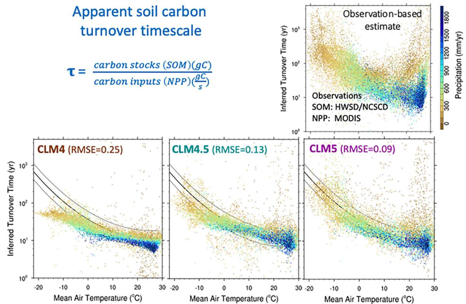
Figure 12. Metric for apparent soil carbon turnover time versus mean air temperature, as in Koven et al. (2017) for observations and CLMBGC model versions. Turnover time is calculated in observations and models as ratio of mean carbon stocks (SOM) over climatological annual mean carbon inputs (NPP). Each dot represents one grid cell, color coded by mean annual precipitation. The best fit regression curve for the observational data with 50% prediction intervals is shown as black lines for the models. RMSE represents the agreement with the best fit curves. See Koven et al. (2017) for full description of this metric. Observations for soil organic matter (SOM) are merged from Harmonized World Soil Database (Fao/Iiasa/Isric/Isscas/Jrc, 2012) and Northern Circumpolar Soil Carbon Database (Hugelius et al., 2013). Observed NPP estimate is from MODIS (Zhao et al., 2005).
