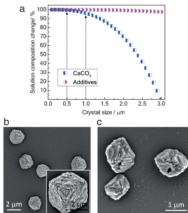
Figure 3. a) Estimated change in the solution composition during crystallization from a solution with [\text{Ca}^{2+}] = 2.5 \text{ mM} and [\text{PSS}] = 250 \mu\text{g mL}^{-1} . b, c) Crystals grown from 1–3 \mu\text{m} calcite seed crystals in a continuous-flow cell from a solution with a constant composition of [\text{Ca}^{2+}] = 3.2 \text{ mM} , [\text{HCO}_3^-] = 6.4 \text{ mM} , [\text{NaCl}] = 35 \text{ mM} , and [\text{PSS}] = 250 \mu\text{g mL}^{-1} . Ionic strength = 0.05 mM, pH 8.5, SI = 1.4.
