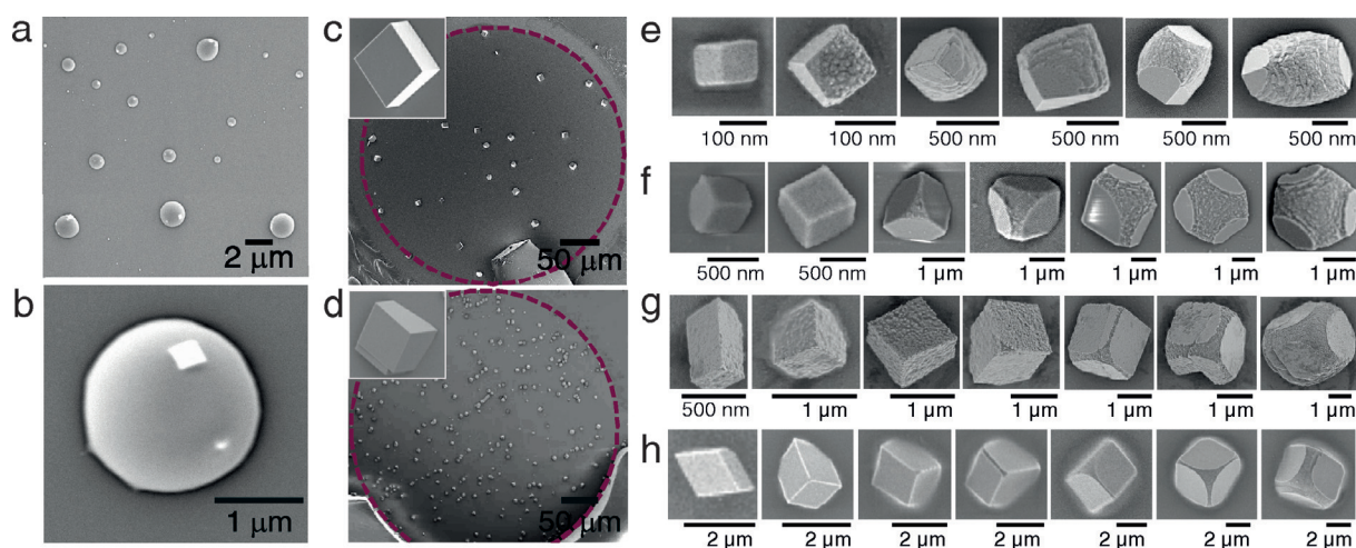
Figure 2. SEM images of \text{CaCO}_3 precipitates in the Crystal Hotel. a, b) Amorphous calcium carbonate obtained at [\text{Ca}^{2+}] = 2.5\ \text{mM} and [\text{Mg}^{2+}] = 1.25\ \text{mM} . Further images of ACC precipitated under a range of solution conditions are shown in Figures S3 and S4. c, d) Calcite crystals grown without additives at [\text{Ca}^{2+}] = 5\ \text{mM} and [\text{Ca}^{2+}] = 50\ \text{mM} , respectively. The purple dotted line indicates the boundaries of the individual “room”. The insets show crystals at higher magnifications. e–h) Crystals formed in the presence of e) [\text{Ca}^{2+}] = 2.5\ \text{mM} and [\text{Mg}^{2+}] = 1.25\ \text{mM} , f) [\text{Ca}^{2+}] = 2.5\ \text{mM} and [\text{PSS}] = 500\ \mu\text{g mL}^{-1} , g) [\text{Ca}^{2+}] = 2.5\ \text{mM} and [\text{PSS}] = 250\ \mu\text{g mL}^{-1} , and h) [\text{Ca}^{2+}] = 1.25\ \text{mM} and [\text{PSS}] = 250\ \mu\text{g mL}^{-1} .
