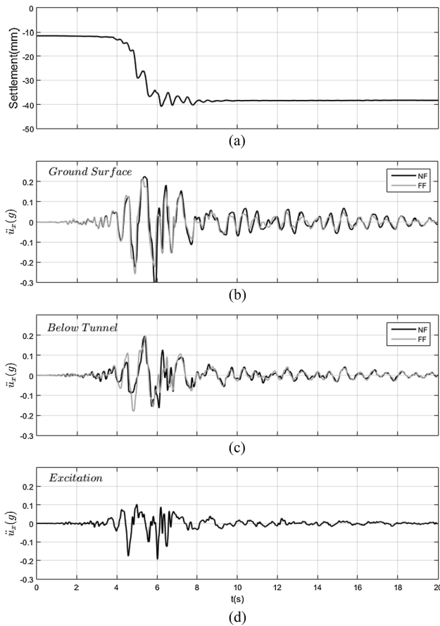
Fig. 6. Tunnel subjected to TK-0.2 g seismic excitation, D_r = 60\% , c' = 0\text{kPa} , V_L = 0\% . Time histories of: (a) settlement at the ground surface above the tunnel crown; (b) near-field (NF) and free-field (FF) horizontal acceleration, \ddot{u}_x , at the ground surface above the tunnel crown; (c) near-field (NF) and free-field (FF) horizontal acceleration below the tunnel; and (d) seismic excitation.
