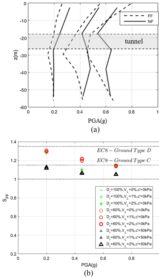
Fig. 9. (a) Near-field (NF) and free-field (FF) peak acceleration profile with depth z ; (b) FF amplification factors, S_{FF} , varying with PGA for D_r = 60\% , 100\% , V_L = 0\% , 1\% , 2\% and c' = 0\text{kPa} , 50\text{kPa} .
