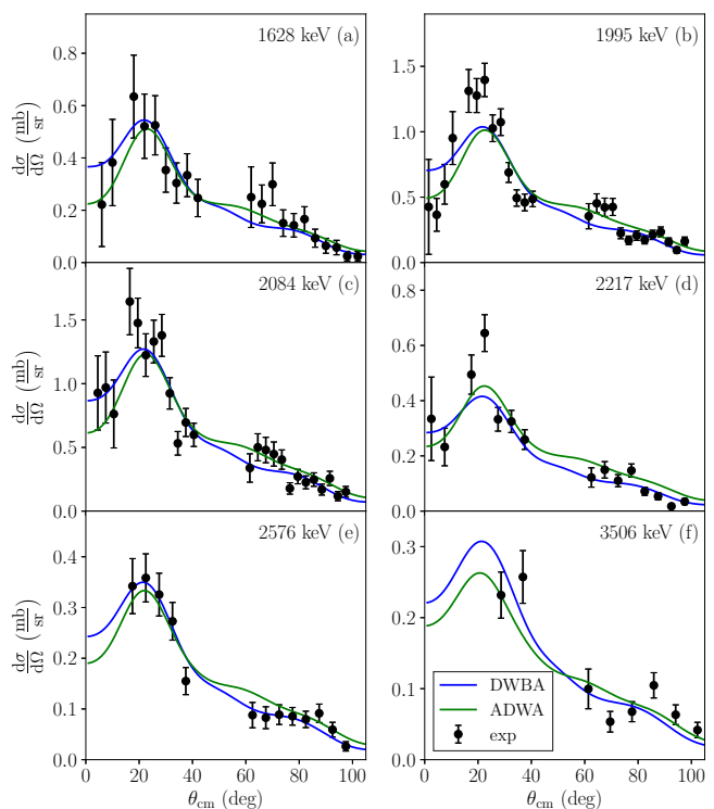
FIG. 10. Angular distributions for \Delta\ell = 2 states in ^{96}\text{Sr} . The experimental data is presented alongside the fitted DWBA (blue) and ADWA (green) calculations, respectively.
