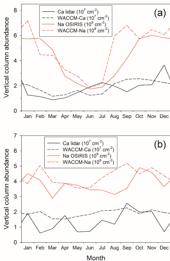
Figure 6: Comparison of observed and modelled Ca and Na vertical column abundances: (a) at Kühlungsborn (54° N); (b) at Arecibo (18° N). The Na column observations were made with the Osiris spectrometer on the ODIN satellite (Fan et al., 2007).
