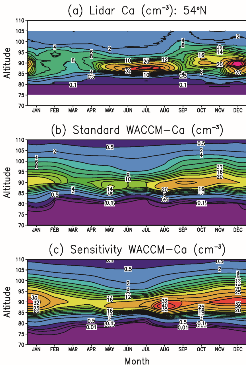
Figure 5: Annual variation of the Ca layer over Kühlungsborn ( 54^\circ\text{N} ): (a) lidar measurements; (b) WACCM-Ca standard model run; (c). WACCM-Ca sensitivity run where the rate coefficients for R24 and R25 are set to their respective Langevin capture rates.
