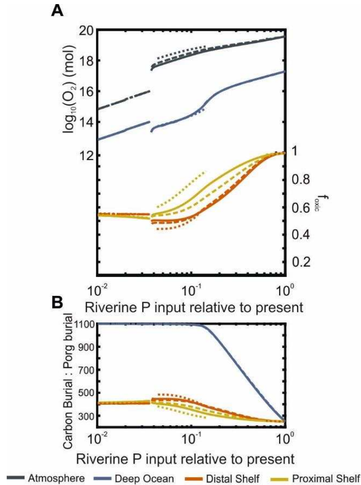
Figure S1. Steady state responses with varying riverine P input relative to present. The f_{oxic} parameter is used to quantify the percentage of anoxic sea floor and is quantified by 1 - f_{anoxic} , as described in the model ( f_{anoxic} = 0.0025 present day; Watson et al., 2017). Varying redox dependencies on P_{org} and P_{auth} burial are shown for values used in previous models of Slomp and Van Cappellen, 2007 (10% - P_{auth} and 10% - P_{org} ) (solid line). Greater redox dependencies are also tested (25% - P_{auth} and 50% - P_{org} , dashed line; 90% - P_{auth} and 50% - P_{org} , dotted line). Regions in which lines do not continue indicate unstable model outputs.
