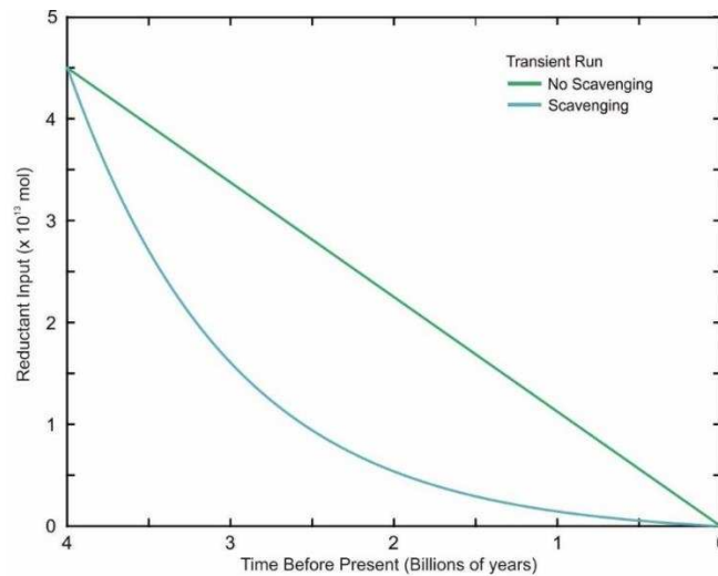
Figure S3. Estimated flux of O 2 consumption via reductant input. Green line follows the linear decreasing trend through time, used for the transient run that did not included scavenging in Figure 5. Blue line follows an approximately exponential decrease used for the transient run that did included scavenging in Figure 5.
