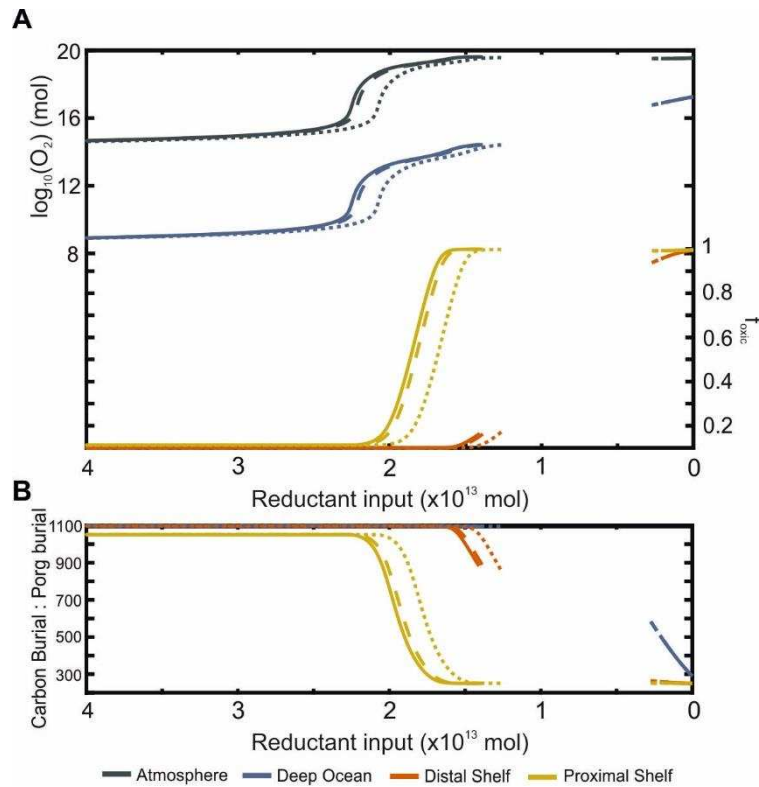
Figure S2. Steady state responses with varying reduced gas concentrations with the inclusion of the scavenging flux. (A) The f_{\text{oxic}} parameter is used to quantify the percentage of anoxic sea floor and is quantified by 1 - f_{\text{anoxic}} , as described in the model ( f_{\text{anoxic}} = 0.0025 present day; Watson et al., 2017). Redox dependencies are set to values from Slomp and Van Cappellen (2007), where 50% of P_{\text{auth}} and 25% of P_{\text{org}} are redox dependent. (B) Carbon and phosphorus burial ratio in sediments. Breaks in solid lines indicate periods where no stable solution exists, in these parameter spaces the model produces an oscillating solution. (No scavenging, solid line; maximum value of 1 \times 10^9 mol P/yr, dashed line; maximum value of 5 \times 10^9 mol P/yr, dotted line).
