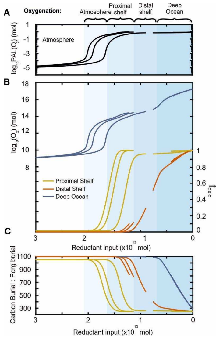
Figure 3. Model stable solutions with respect to overall surface redox state. The model is run to steady state for changes to the reduced gas input rate. (A) Atmospheric O_2 reservoir. (B) Deep ocean O_2 reservoir (mol) and shelf 'oxic fraction' of seafloor ( f_{oxic} ). (C) Molar carbon and phosphorus burial ratio in sediments. Three lines for each zone represent different choices of redox dependence for P burial fluxes (see text). Breaks in solid lines indicate periods where no stable solution exists, in these parameter spaces the model produces an oscillating solution.
