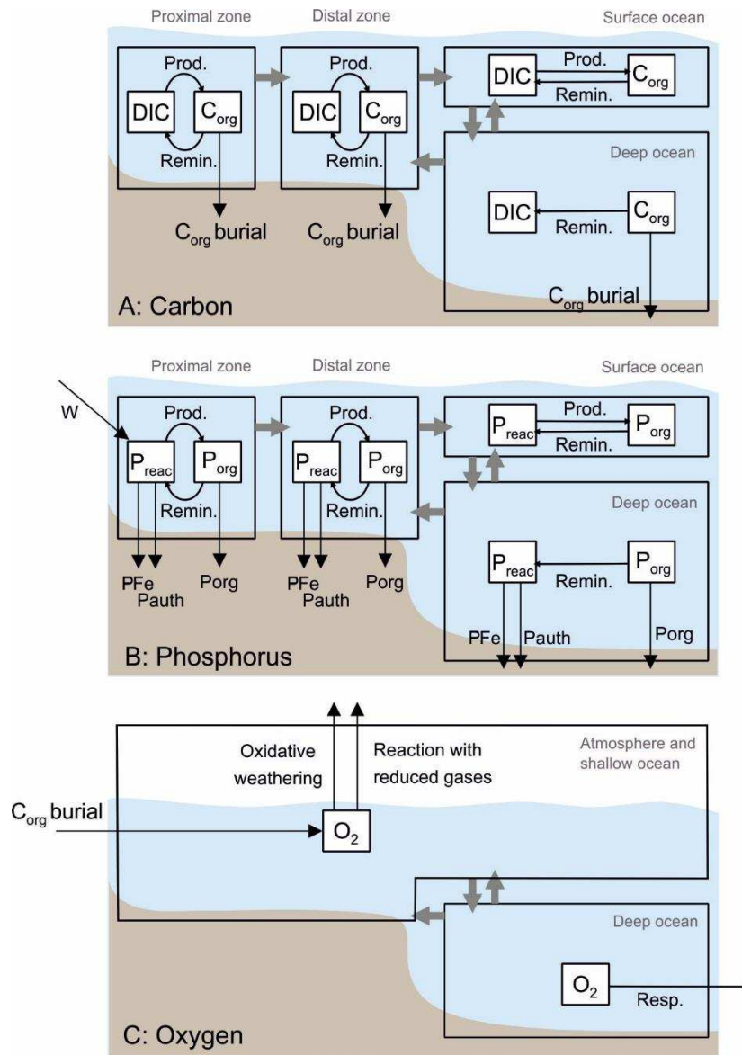
Figure 2. Ocean and atmosphere box model. Clear boxes show hydrographic reservoirs and grey arrows denote mixing between them. White boxes show chemical reservoirs and black arrows denote biogeochemical fluxes. (A) Carbon cycle: C exists as dissolved inorganic carbon (DIC) or organic carbon (C org ). (B) Phosphorus cycle: P exists as soluble reactive phosphorus (P react ) and particulate organic phosphorus (P org ). (C) Oxygen cycle. Single oxygen reservoir encompasses all ocean boxes that exchange with the atmosphere. See text for full description, and methods and SI for equations.
