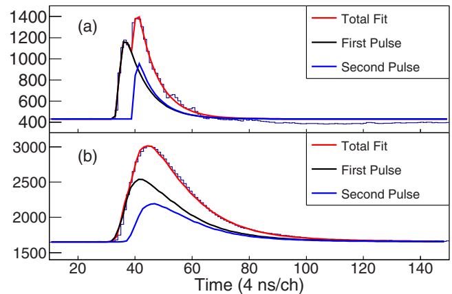
FIG. 2. Typical recorded traces of successive decays with rise time of 10 ns and time interval of 17 ns dynode signal and corresponding anode signals are shown in (a) and (b) respectively. Anode pileup pulses with slow rise time can be decomposed using the timing information from the dynode and fitted averaged anode pulses.
