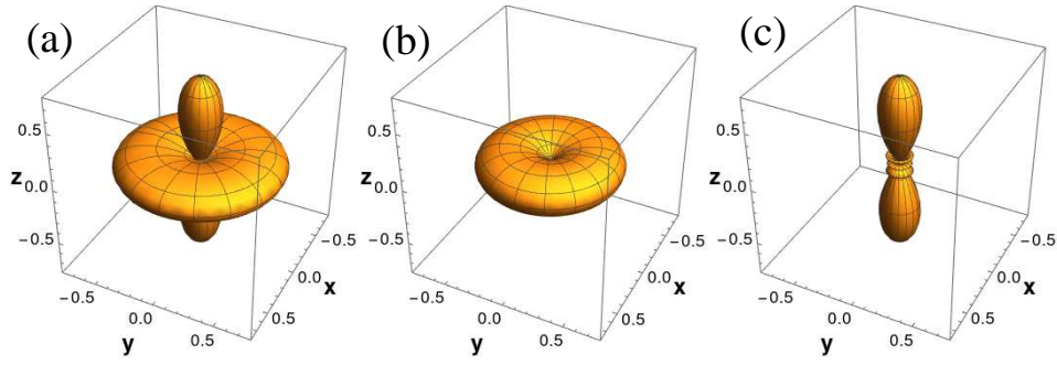
FIG. 1: d^*(2380) quadrupole deformation produced by N\Delta\pi ((b), B -term), middle; double-pionic cloud ((c), C -term), right and total effect, left, (a).
