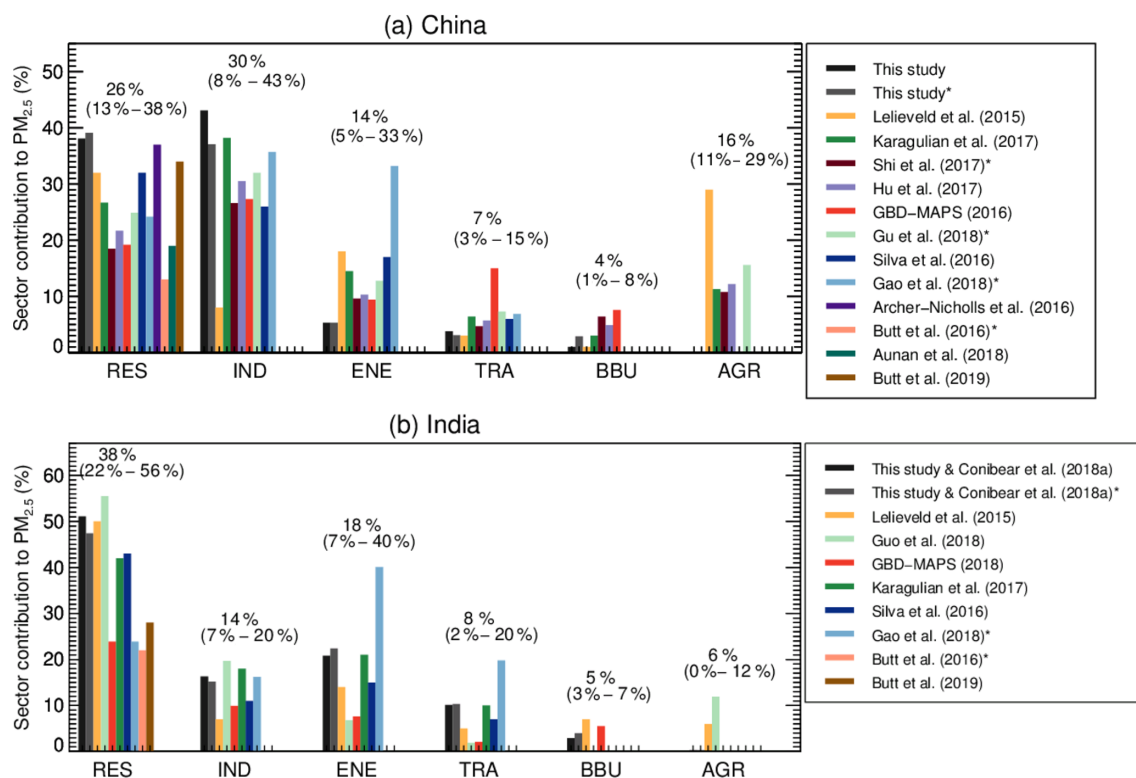
Figure 7. Comparison of relative sector-specific contributions to annual mean PM 2.5 concentrations in (a) China and (b) India from this study and previous studies. Bars show sector contributions to population-weighted annual mean PM 2.5 concentrations, with the exception of the bars associated with studies shown in the legend with an asterisk (*), which show estimated sector contributions to surface area-weighted annual mean PM 2.5 concentrations. In our study, population-weighted and area-weighted values differ by less than six percentage points. The mean relative contribution of each sector is shown above the bars with the range of values (minimum to maximum) in parentheses. The values for each study are also shown in Tables 4 and 5. The emission sectors are agriculture (AGR), power generation (ENE), industrial non-power (IND), residential energy use (RES), land transport (TRA), and open biomass burning (BBU). We note that the contribution of the agricultural section to PM 2.5 is not quantified for China in this study.
