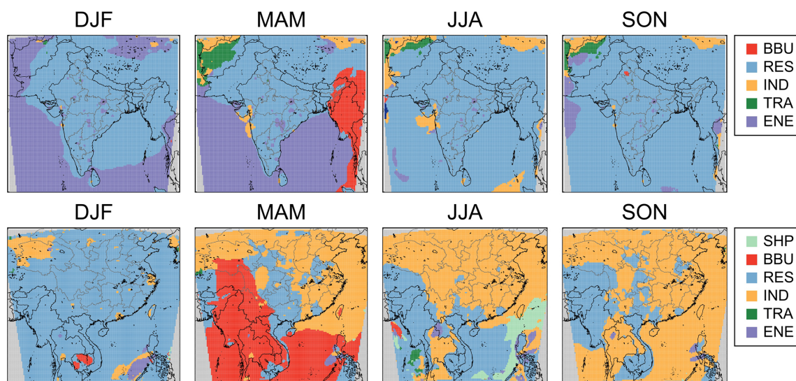
Figure 5. Spatial distribution of the dominant anthropogenic emission sectors for seasonal mean PM 2.5 in South Asia (top panel) and East Asia (bottom panel). DJF: December, January, February mean; MAM: March, April, May mean; JJA: June, July, August mean; SON: September, October, November mean. As for Fig. 4, the dominant emission sector is calculated for each model grid cell as the emission sector that gives the largest reduction in simulated seasonal mean surface PM 2.5 concentration, i.e. results in the largest absolute difference in \mu\text{g m}^{-3} from the control simulation. Regions in grey are outside the model domain. The emission sectors shown are power generation (ENE), industrial non-power (IND), residential energy use (RES), land transport (TRA), open biomass burning (BBU), and shipping (SHP; East Asia only).
