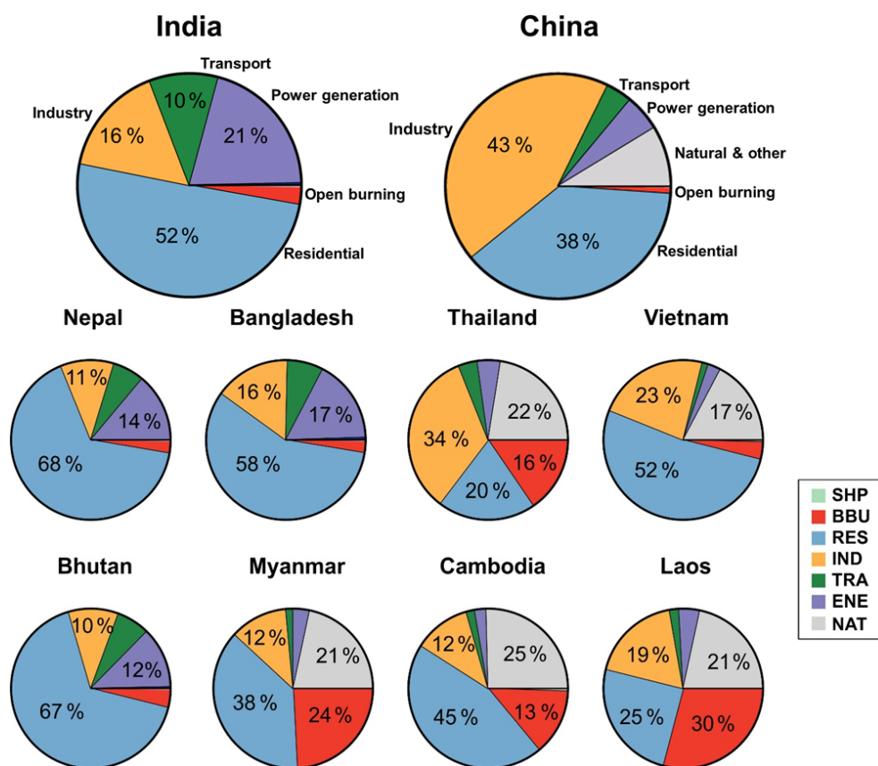
Figure 2. Relative contributions of different anthropogenic emission sectors to population-weighted annual mean PM 2.5 concentration by country in South and East Asia. Emission sectors include agriculture (AGR; South Asia only), power generation (ENE), industrial non-power (IND), residential energy use (RES), land transport (TRA), open biomass burning (BBU), and shipping (SHP; China and mainland South-east Asia only). Where the percentage contributions from each sector do not add up to 100 %, the residual fraction is assigned to “Natural and other sources” (NAT). Sectors are listed in the legend only if their contribution is visible in the pie charts. Relative contribution values of 10 % or greater are shown in the quadrants. Results are shown for the region of China contained within the model domain, which accounts for 92 % of the Chinese population (Sect. 2.2).
