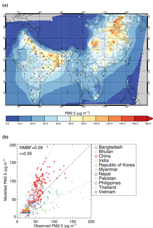
Figure 1. Simulated and measured annual mean surface PM 2.5 concentrations across South and East Asia. Observation data are from the World Health Organization database, 2016 and 2018. (a) Map of the simulated surface distribution of annual mean PM 2.5 for 2014 (underlying colours); overlying circles show measured annual mean PM 2.5 concentrations for available years (2009–2016). Regions in grey are outside the model domain. (b) Simulated versus measured annual mean PM 2.5 concentrations. Circles show measured annual mean PM 2.5 concentrations for the year 2014; diamonds show measured annual mean PM 2.5 concentrations for years other than 2014. All simulated annual mean PM 2.5 concentrations are for the year 2014. The normalized mean bias factor (NMBF; Yu et al., 2006) and Pearson's correlation coefficient ( r ) between simulated and measured values are displayed in the top left corner.
