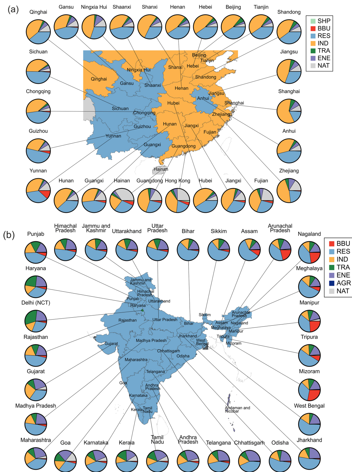
Figure 3. Contribution of different emission sectors to population-weighted annual mean PM 2.5 concentration (a) by province/municipality/region in China and (b) by state in India (Union Territories are not shown individually, apart from Delhi National Capital Territory (NCT)). The colour of each province in China and each state in India indicates the sector that dominates contributions to population-weighted annual mean PM 2.5 in that province or state. The emission sectors are agriculture (AGR; India only), power generation (ENE), industrial non-power (IND), residential energy use (RES), land transport (TRA), open biomass burning (BBU), and shipping (SHP; China only). Where the percentage contributions from each sector do not add up to 100%, the residual fraction is assigned to “Natural and other sources” (NAT).
