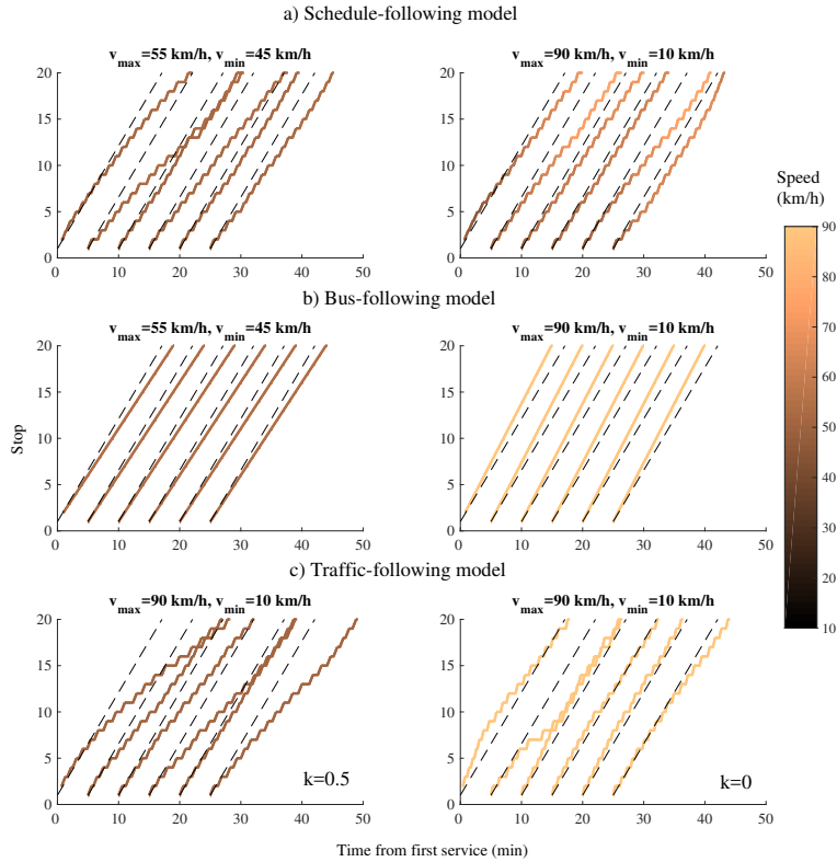
Figure 5.: Impact of speed constraints on on-time performance: (a) schedule-following model, (b) bus-following model, and (c) traffic-following model
