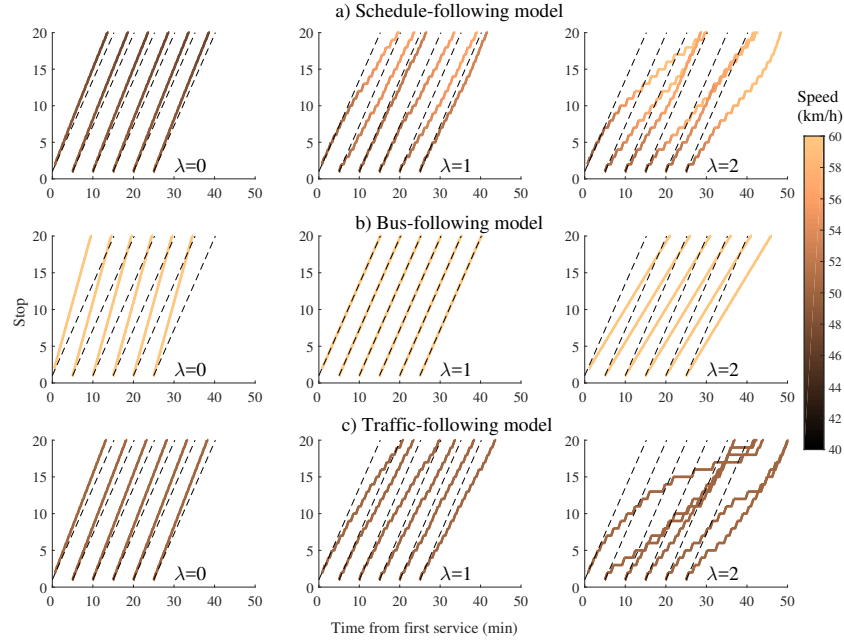
Figure 4.: Sensitivity of \lambda : (a) schedule-following model, (b) bus-following model, and (c) traffic-following model
