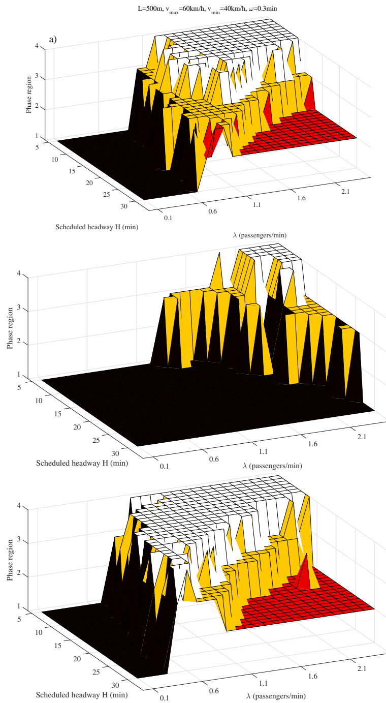
Figure 8.: Phase diagram analysis of: (a) schedule-following model, (b) bus-following model, and (c) traffic-following model under small perturbation
