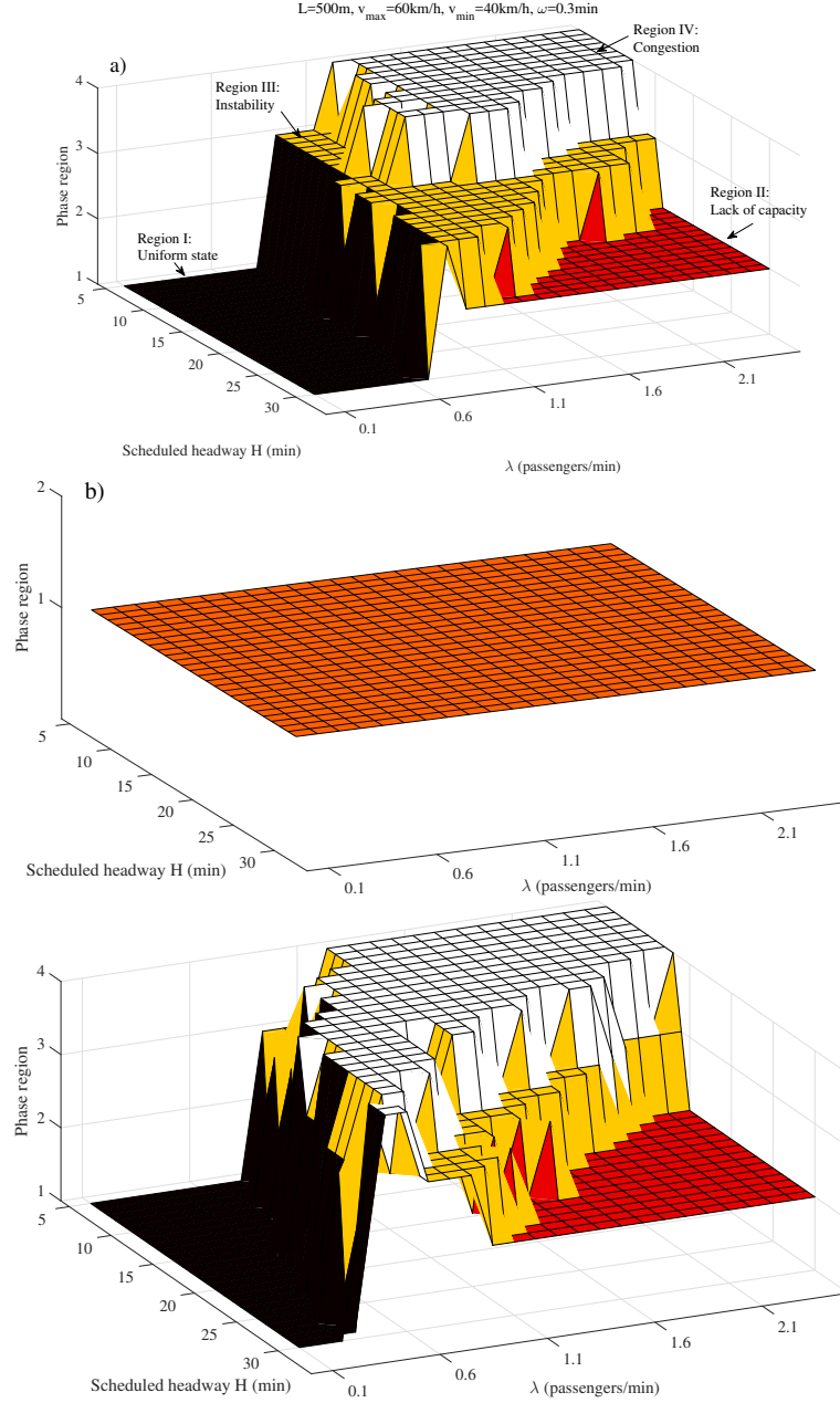
Figure 6.: Phase diagram analysis of: (a) schedule-following model, (b) bus-following model, and (c) traffic-following model
