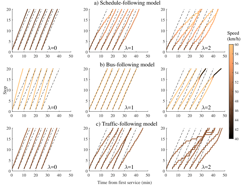
Figure 7.: Bus trajectories after random perturbations:(a) schedule-following model, (b) bus-following model, and (c) traffic-following model
