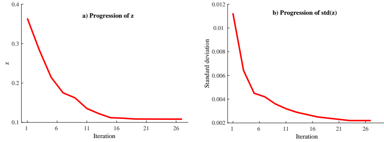
Figure 9.: Progression of the performance index z (over 1000 samples): (a) Convergence of the mean of z , (b) Convergence of the standard deviation of z
