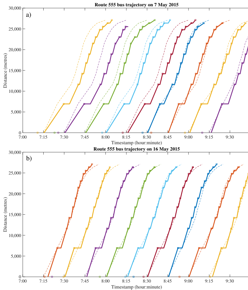
Figure 1.: Observed bus trajectories (bold line) compared with the schedule (dashed line) from:(a) weekday, b) weekend
