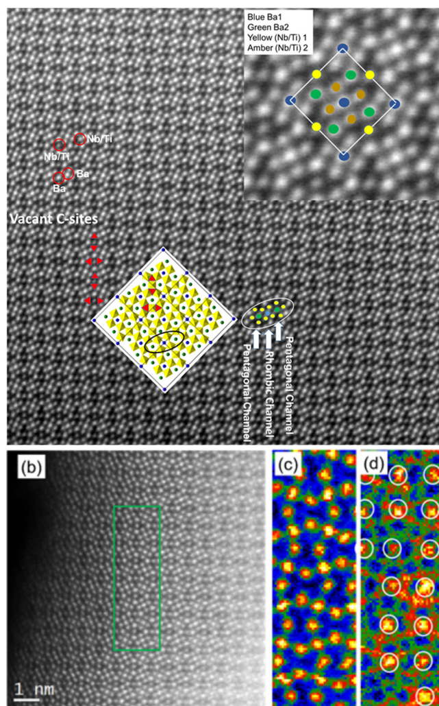
FIG. 3. [001] HAADF image and EELS data for BTN-S ceramic. (a) Top right inset is the superimposition of the proposed crystal structure obtained by XRD on the HAADF image. (b) HAADF image with the green rectangle showing the area used for chemical analysis. (c) and (d) EELS maps for Ba and Ti, respectively.
