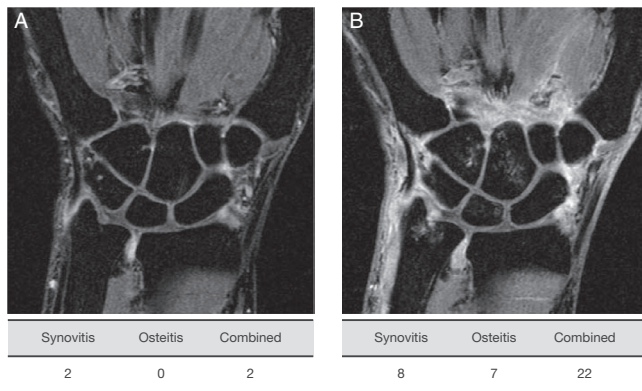
Figure 1. Contrast-enhanced 1.5T magnetic resonance image (MRI) of wrist with low (A) and high (B) MRI-detected inflammation. Low MRI inflammation: synovitis \leq 3 or osteitis \leq 3 and combined \leq 9 (synovitis plus 2x osteitis). High MRI inflammation: synovitis >3 and osteitis >3 or combined >9 (synovitis plus 2x osteitis).
