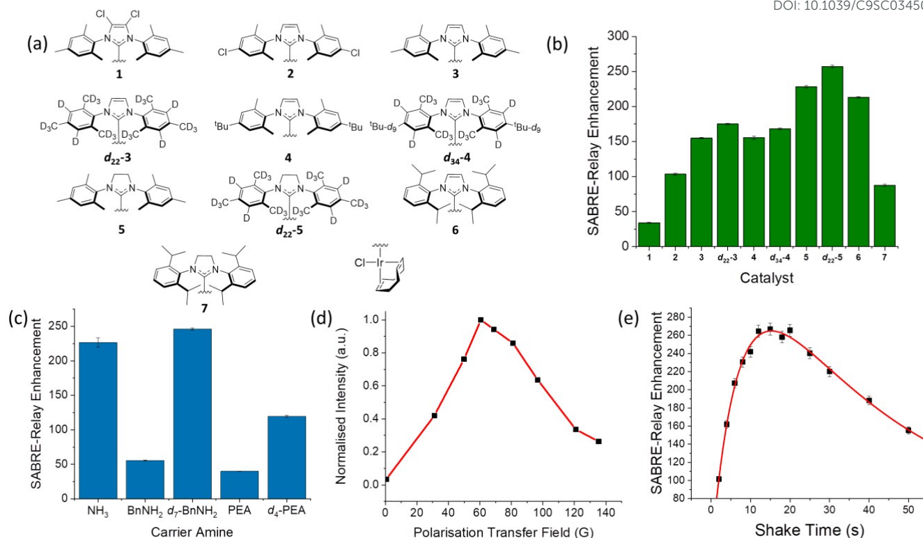
Figure 6 - (a) Structures of the ten different catalysts used in collecting the SABRE-Relay 13 C signal enhancements for D-glucose- 13 C 6 - d 7 shown in (b); the largest enhancement was observed for d 22 -5. (c) Corresponding 13 C signal enhancement factors achieved using pre-catalyst d 22 -5 and the indicated NH containing materials ammonia (NH 3 ), benzylamine (BnNH 2 ), benzyl- d 7 -amine ( d 7 -BnNH 2 ), phenethylamine (PEA) and phenethyl-1,1,2,2- d 4 -amine ( d 4 -PEA); all samples contained 10.3 mM of the NH source and 4.8 mM of d 22 -5 in a DCM- d 2 : DMF (1.6:1) solution that was shaken at 60.6 G for ten seconds. (d) Polarization transfer field dependence on the signal gain for a D-glucose- 13 C 6 - d 7 sample with 4.8 mM of 3 in a DCM- d 2 : DMF (1.6:1) solution measured at 1 T; PTF obtained using a set of bespoke Halbach arrays. 69 (e) Signal gain as a function of shake time for a D-glucose- 13 C 6 - d 7 sample using 4.8 mM of d 22 -5 in a DCM- d 2 : DMF (1.6:1) solution; a bi-exponential equation was used to fit the data which highlights the process of polarization build up versus p -H 2 consumption in the NMR tube.
