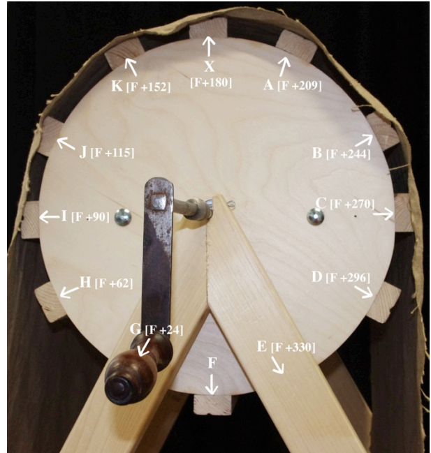
Figure 2: Side view of the acoustic wind machine, showing slat positions in a 360° rotation from their position of origin (slat F).
