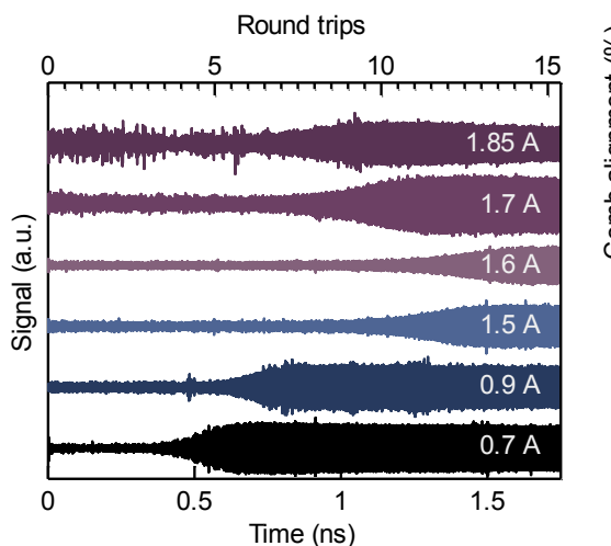
Fig. 3 The electric field from the QCL measured at different current amplitudes in the tuning cavity. The lasing cavity is driven using quasi-dc pulses of amplitude 0.65 A.
