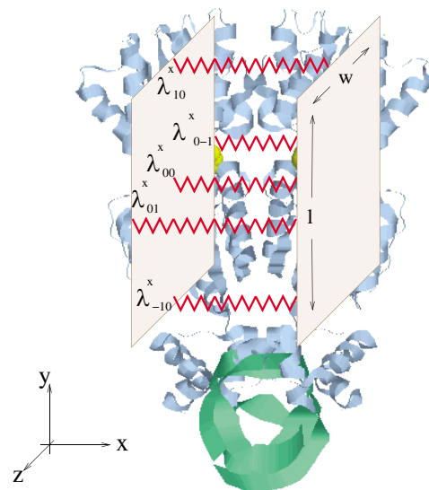
FIG. 1 (color online). Plates and springs model for the interaction of the two domains of a repressor dimer. The x -ray structure (PDB 1EFA [7]) of the lac repressor dimer (with DNA at the bottom) is shown behind the model.
