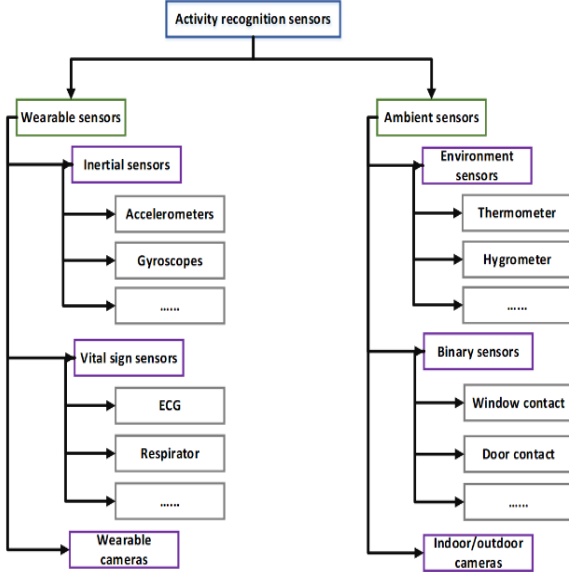
Figure 3. Typical sensors categories for PARM
