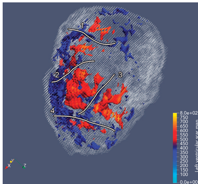
Figure 4: 3D Multiplanar Reconstruction
