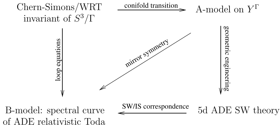
FIGURE 3. The GOV correspondence for S^3/\Gamma .
