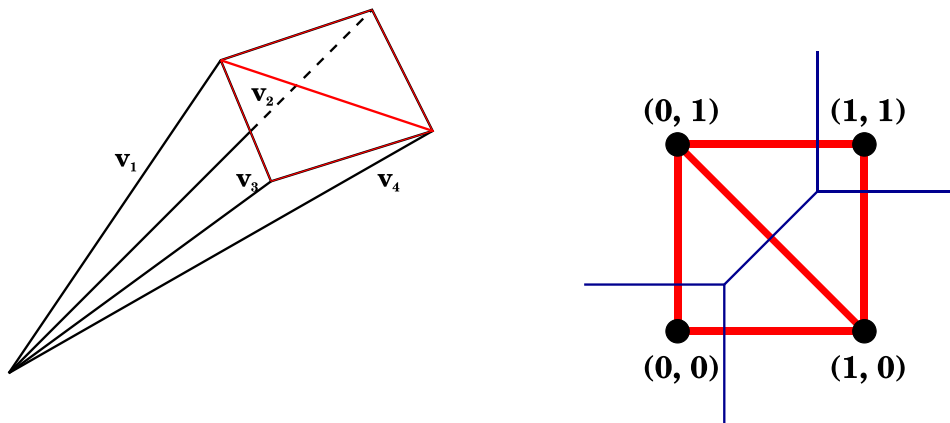
FIGURE 2. The fan (left) of the resolved conifold: its skeleton is given by four rays, labelled v_i in the picture, whose tips lie on an affine hyperplane at unit distance from the origin of \mathbb{Z}^3 . The intersection of the fan with the hyperplane is shown on the right (the toric diagram ); superimposed is the pq-web diagram.
