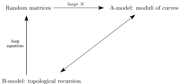
FIGURE 1. Large N duality and mirror symmetry in d = 0
